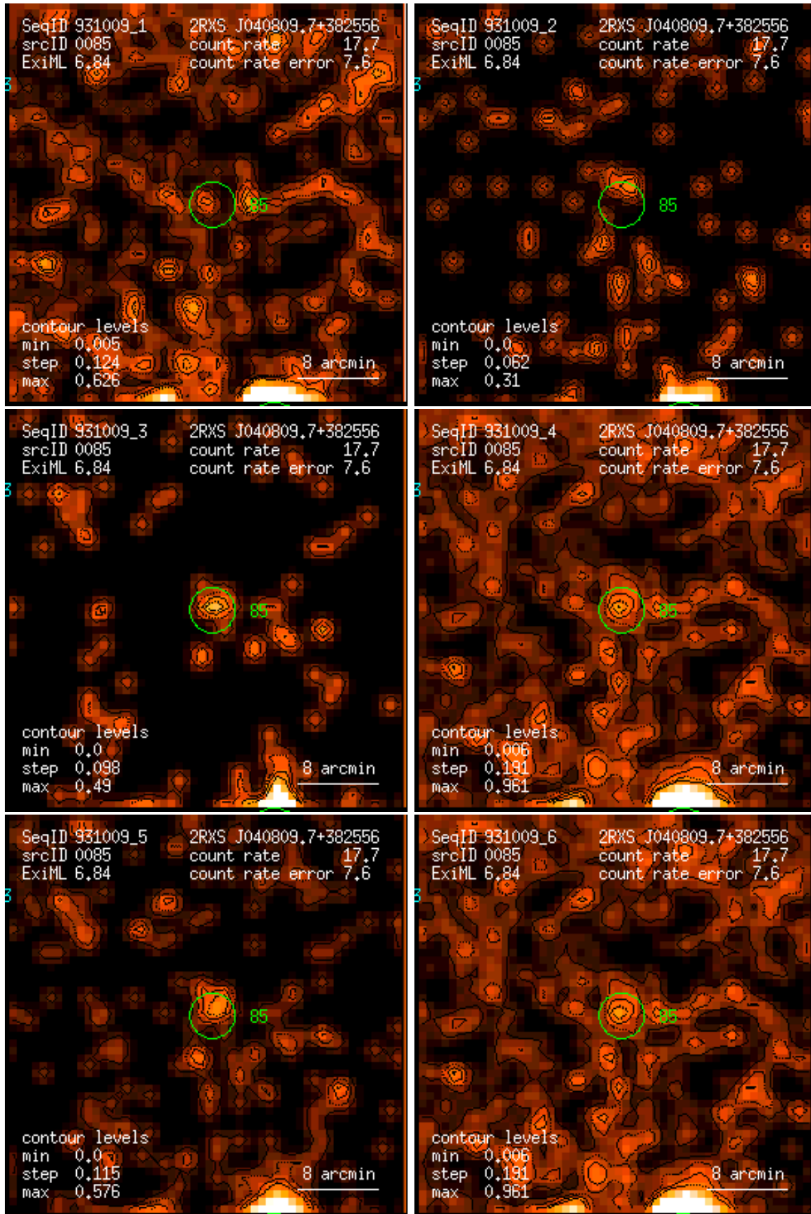
Figure 85: RASS 931009: detection 0085: band rate images, Gaussian filter: (1) PSPC channels 11 – 41, (2) 52 – 90, (3) 91 – 201, (4) 11 – 235, (5) 52 – 201, (6) 11 – 201. Broad band rates in counts/ks. Band rate contour levels in counts/ks/arcmin 2 .
