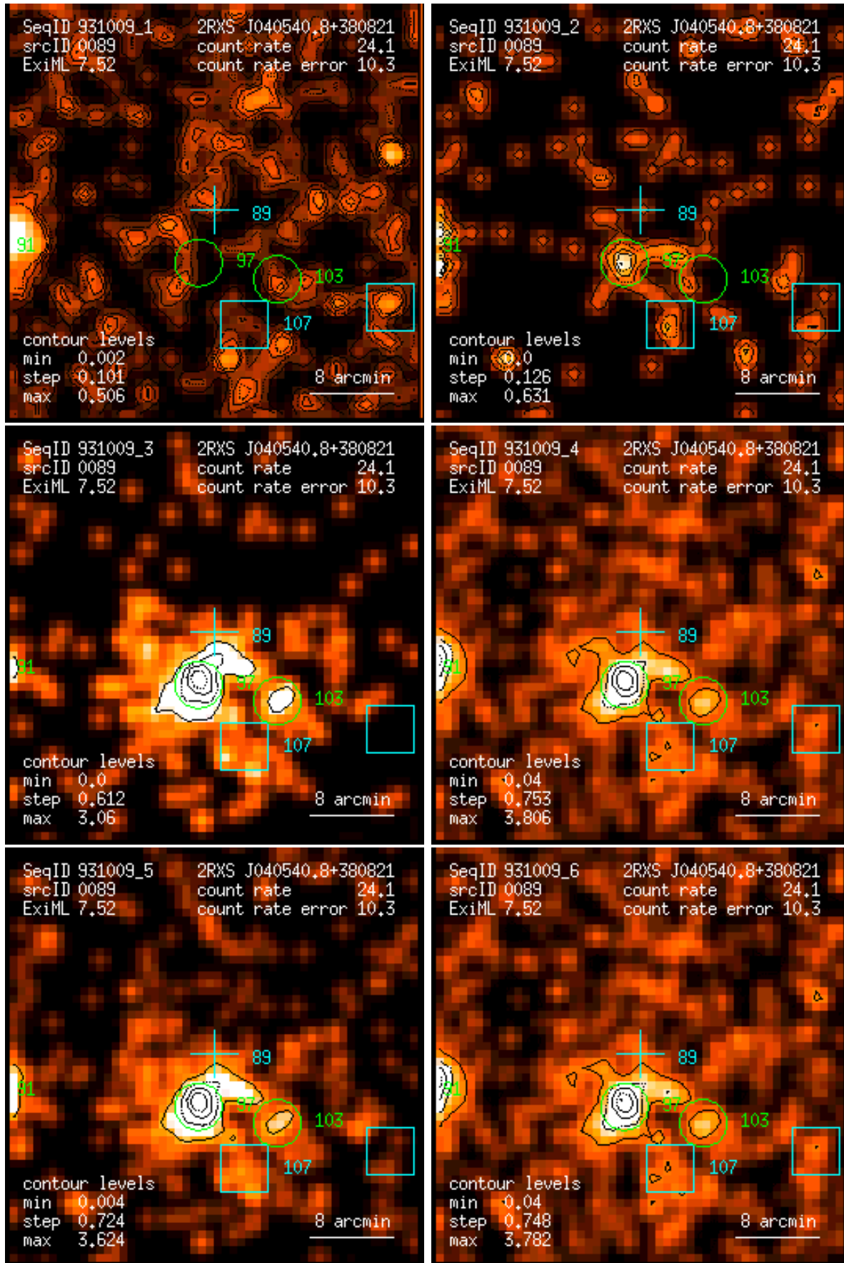
Figure 89: RASS 931009: detection 0089: band rate images, Gaussian filter: (1) PSPC channels 11 – 41, (2) 52 – 90, (3) 91 – 201, (4) 11 – 235, (5) 52 – 201, (6) 11 – 201. Broad band rates in counts/ks. Band rate contour levels in counts/ks/arcmin 2 .
