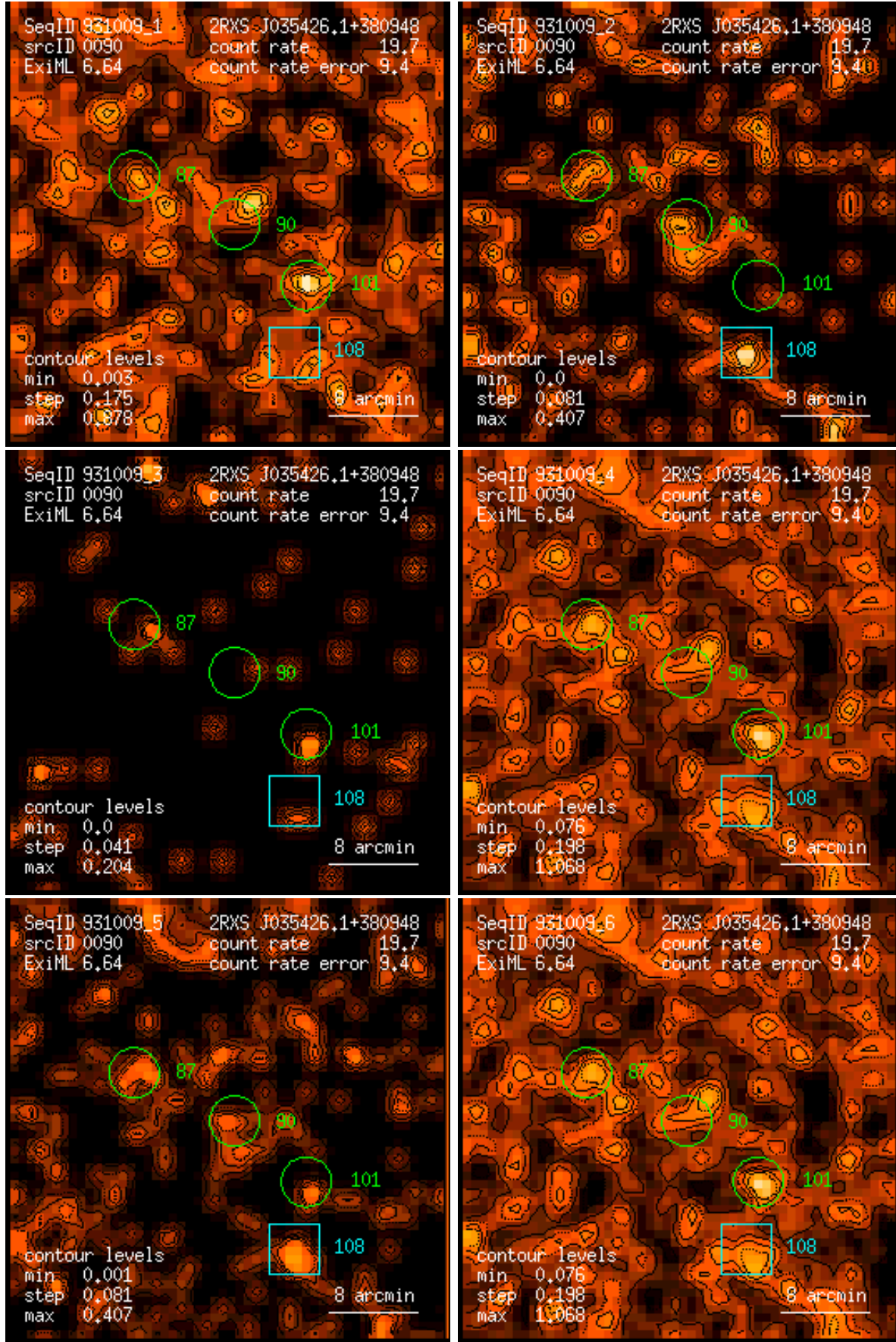
Figure 90: RASS 931009: detection 0090: band rate images, Gaussian filter: (1) PSPC channels 11 – 41, (2) 52 – 90, (3) 91 – 201, (4) 11 – 235, (5) 52 – 201, (6) 11 – 201. Broad band rates in counts/ks. Band rate contour levels in counts/ks/arcmin 2 .
