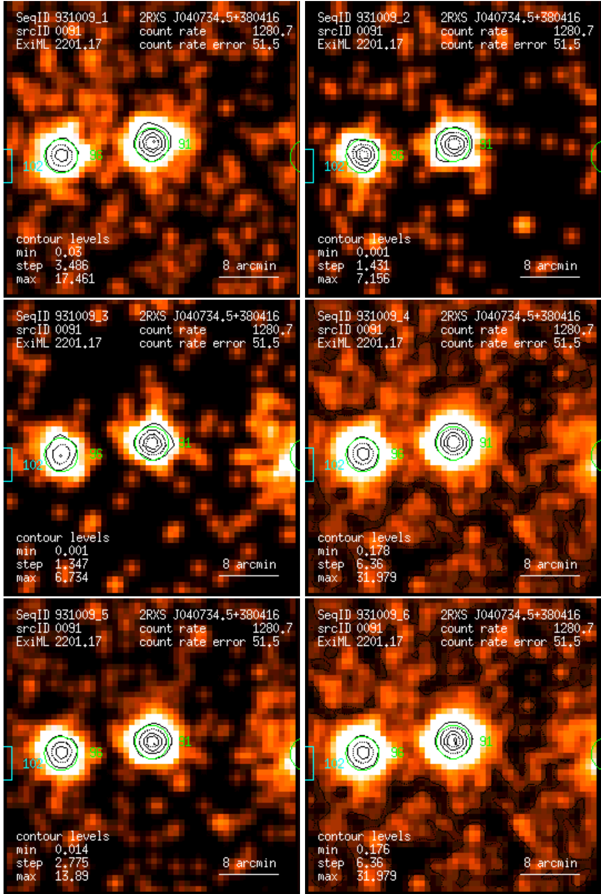
Figure 91: RASS 931009: detection 0091: band rate images, Gaussian filter: (1) PSPC channels 11 – 41, (2) 52 – 90, (3) 91 – 201, (4) 11 – 235, (5) 52 – 201, (6) 11 – 201. Broad band rates in counts/ks. Band rate contour levels in counts/ks/arcmin 2 .
