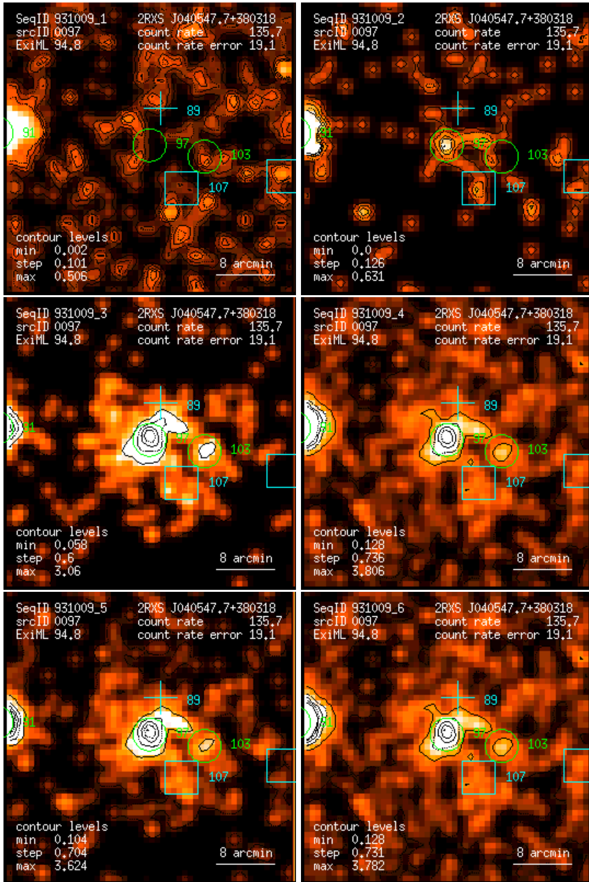
Figure 97: RASS 931009: detection 0097: band rate images, Gaussian filter: (1) PSPC channels 11 – 41, (2) 52 – 90, (3) 91 – 201, (4) 11 – 235, (5) 52 – 201, (6) 11 – 201. Broad band rates in counts/ks. Band rate contour levels in counts/ks/arcmin 2 .
