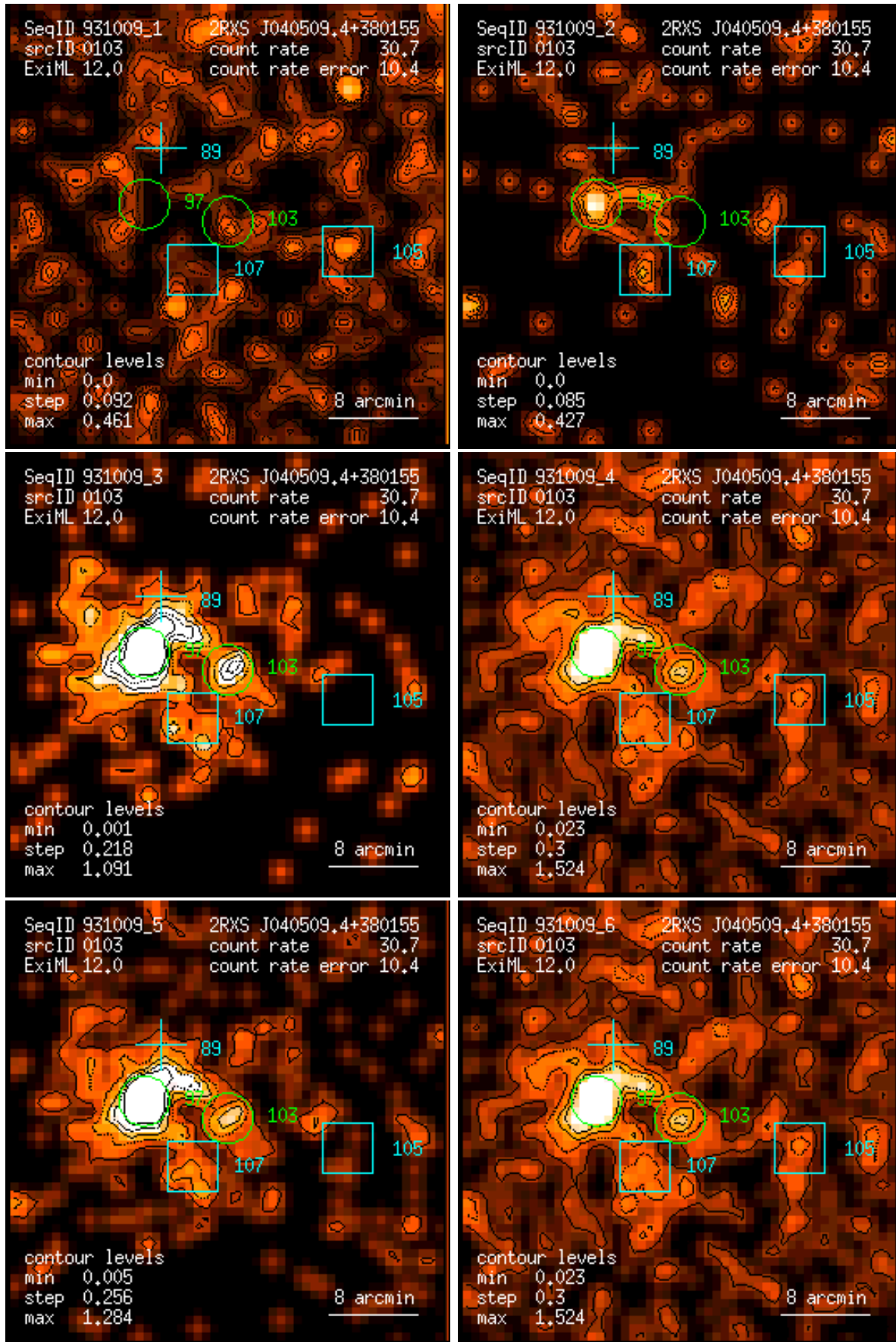
Figure 103: RASS 931009: detection 0103: band rate images, Gaussian filter: (1) PSPC channels 11 – 41, (2) 52 – 90, (3) 91 – 201, (4) 11 – 235, (5) 52 – 201, (6) 11 – 201. Broad band rates in counts/ks. Band rate contour levels in counts/ks/arcmin 2 .
