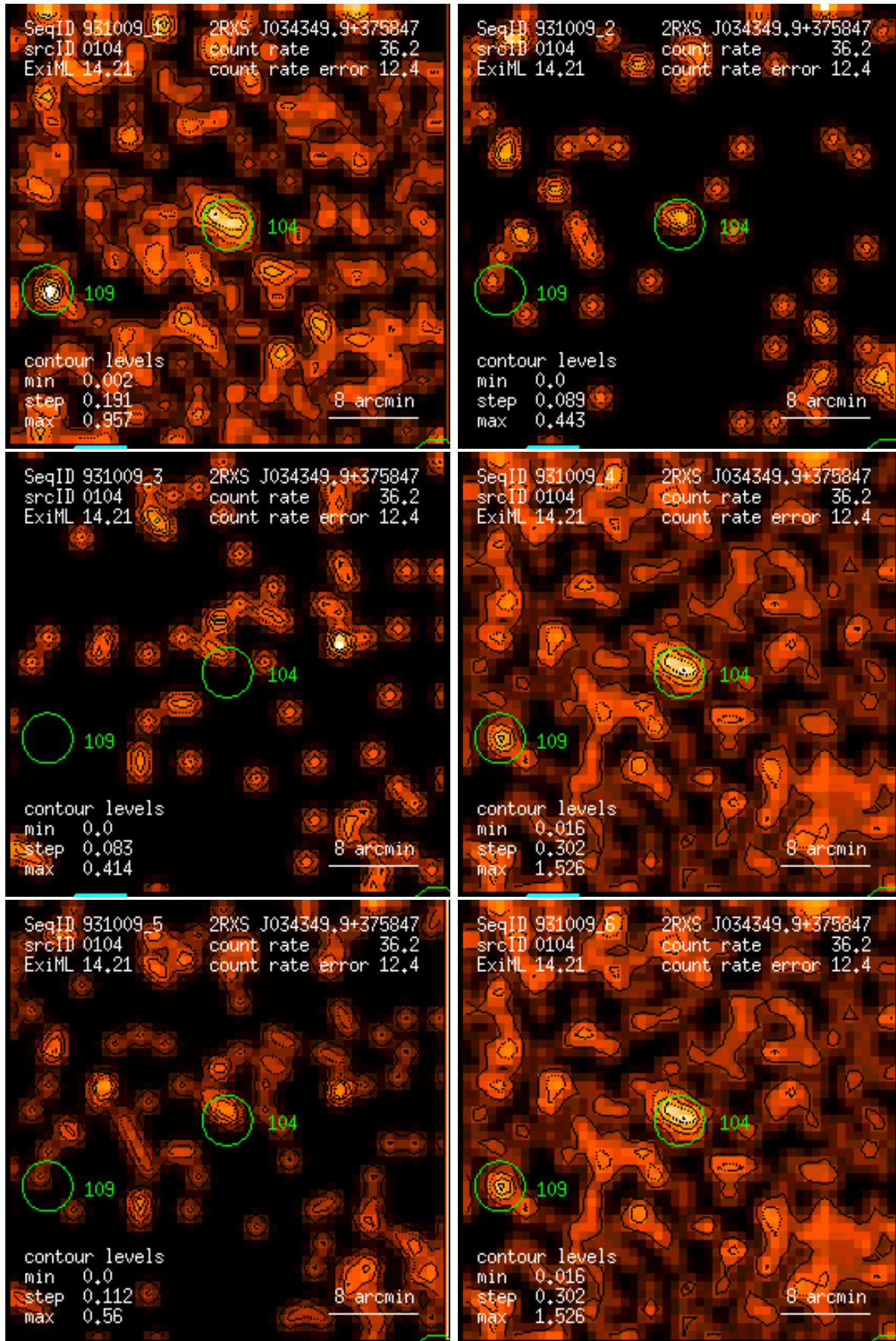
Figure 104: RASS 931009: detection 0104: band rate images, Gaussian filter: (1) PSPC channels 11 – 41, (2) 52 – 90, (3) 91 – 201, (4) 11 – 235, (5) 52 – 201, (6) 11 – 201. Broad band rates in counts/ks. Band rate contour levels in counts/ks/arcmin 2 .
