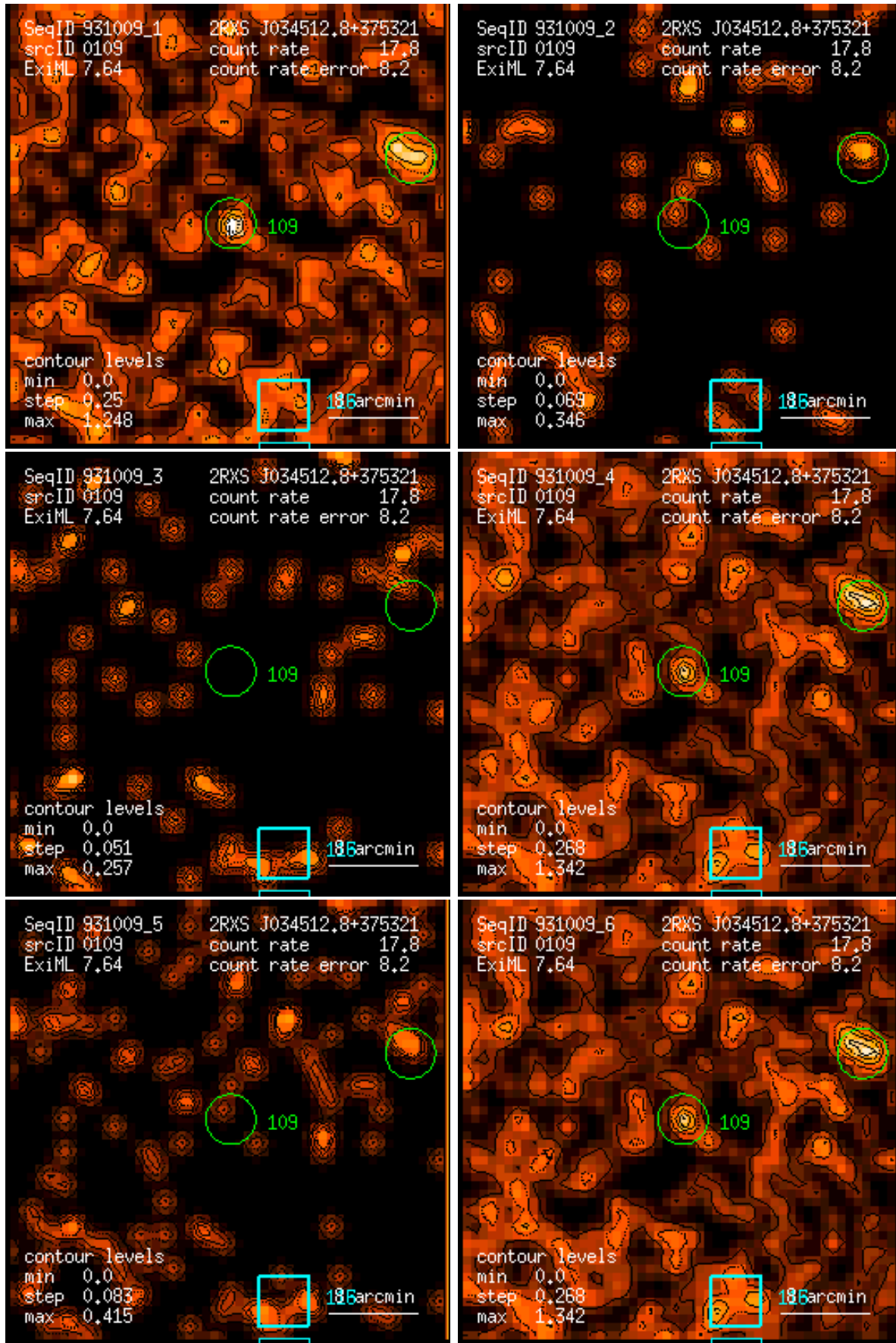
Figure 109: RASS 931009: detection 0109: band rate images, Gaussian filter: (1) PSPC channels 11 – 41, (2) 52 – 90, (3) 91 – 201, (4) 11 – 235, (5) 52 – 201, (6) 11 – 201. Broad band rates in counts/ks. Band rate contour levels in counts/ks/arcmin 2 .
