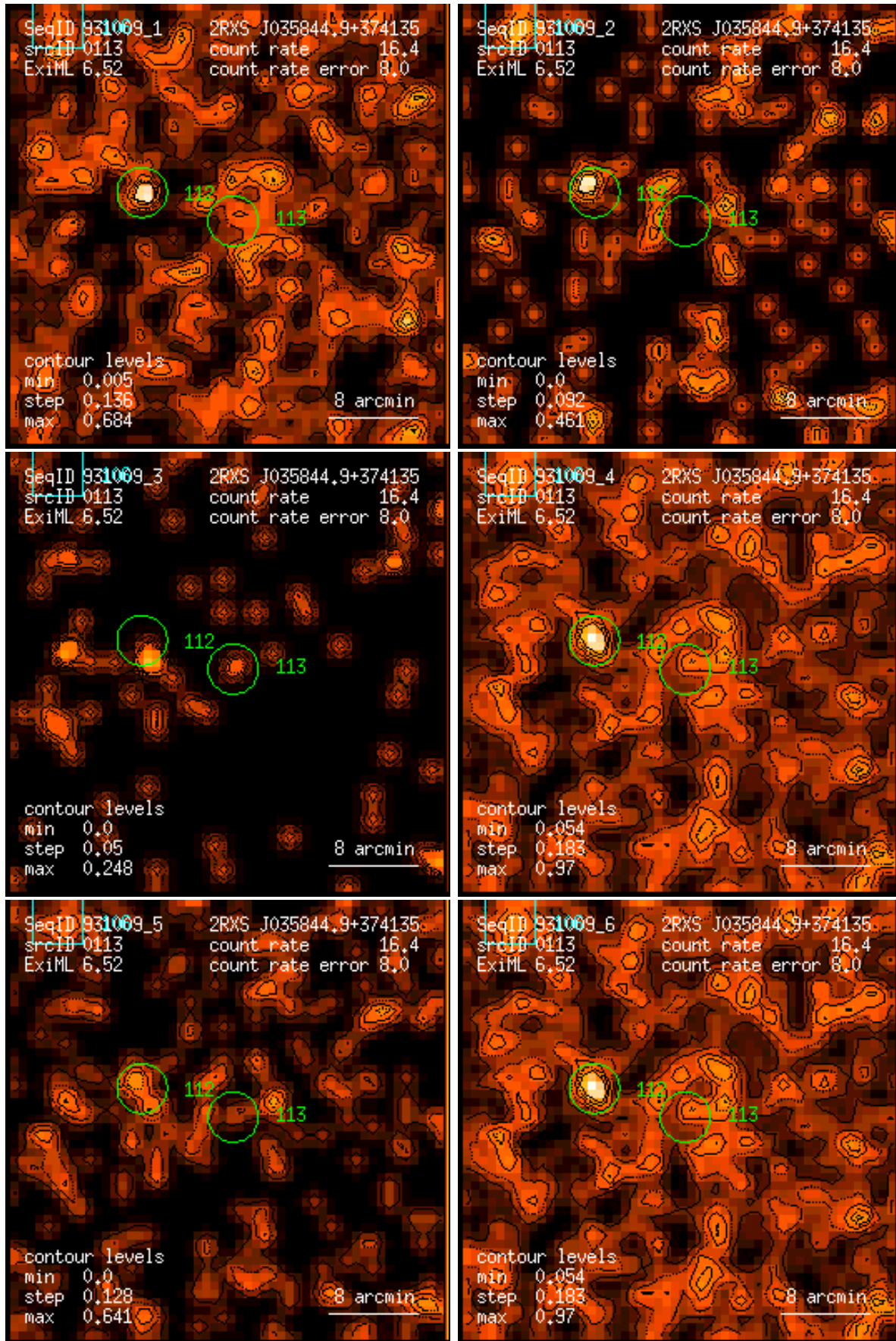
Figure 113: RASS 931009: detection 0113: band rate images, Gaussian filter: (1) PSPC channels 11 – 41, (2) 52 – 90, (3) 91 – 201, (4) 11 – 235, (5) 52 – 201, (6) 11 – 201. Broad band rates in counts/ks. Band rate contour levels in counts/ks/arcmin 2 .
