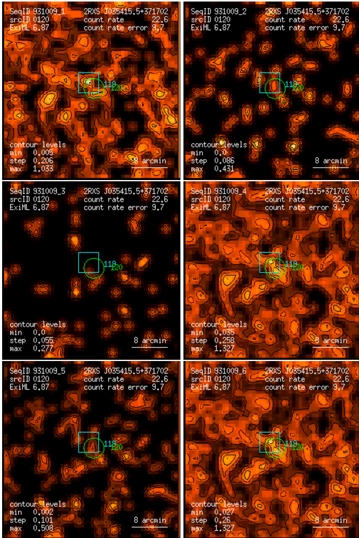
Figure 120: RASS 931009: detection 0120: band rate images, Gaussian filter: (1) PSPC channels 11 – 41, (2) 52 – 90, (3) 91 – 201, (4) 11 – 235, (5) 52 – 201, (6) 11 – 201. Broad band rates in counts/ks. Band rate contour levels in counts/ks/arcmin 2 .
