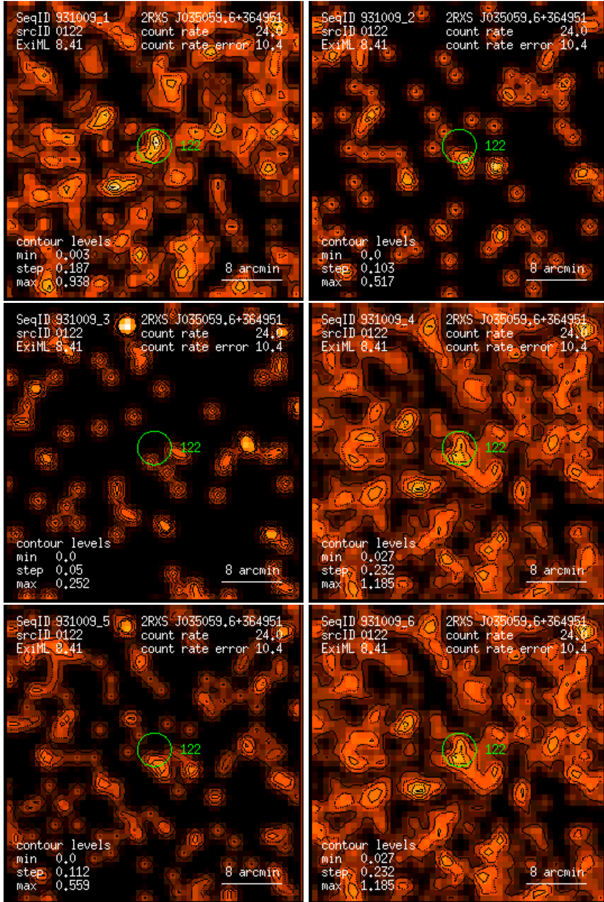
Figure 122: RASS 931009: detection 0122: band rate images, Gaussian filter: (1) PSPC channels 11 – 41, (2) 52 – 90, (3) 91 – 201, (4) 11 – 235, (5) 52 – 201, (6) 11 – 201. Broad band rates in counts/ks. Band rate contour levels in counts/ks/arcmin 2 .
