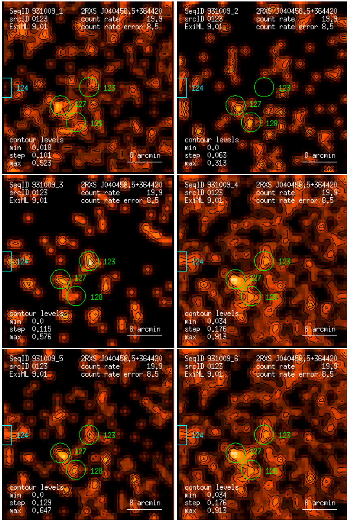
Figure 123: RASS 931009: detection 0123: band rate images, Gaussian filter: (1) PSPC channels 11 – 41, (2) 52 – 90, (3) 91 – 201, (4) 11 – 235, (5) 52 – 201, (6) 11 – 201. Broad band rates in counts/ks. Band rate contour levels in counts/ks/arcmin 2 .
