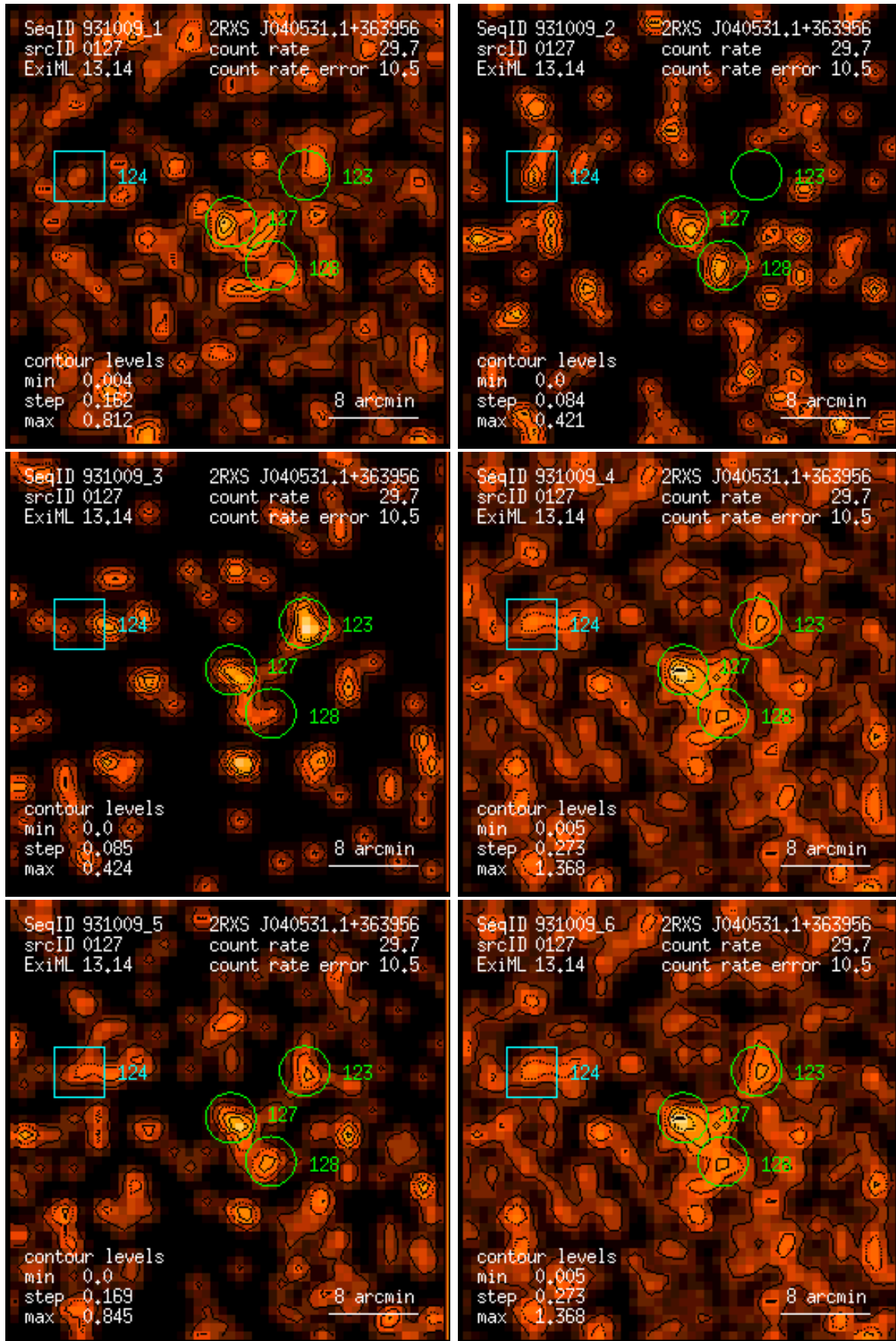
Figure 127: RASS 931009: detection 0127: band rate images, Gaussian filter: (1) PSPC channels 11 – 41, (2) 52 – 90, (3) 91 – 201, (4) 11 – 235, (5) 52 – 201, (6) 11 – 201. Broad band rates in counts/ks. Band rate contour levels in counts/ks/arcmin 2 .
