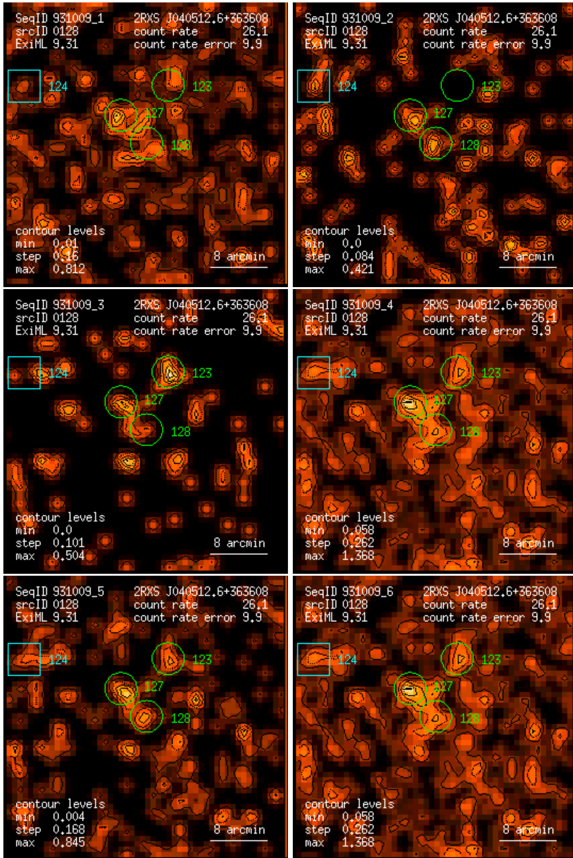
Figure 128: RASS 931009: detection 0128: band rate images, Gaussian filter: (1) PSPC channels 11 – 41, (2) 52 – 90, (3) 91 – 201, (4) 11 – 235, (5) 52 – 201, (6) 11 – 201. Broad band rates in counts/ks. Band rate contour levels in counts/ks/arcmin 2 .
