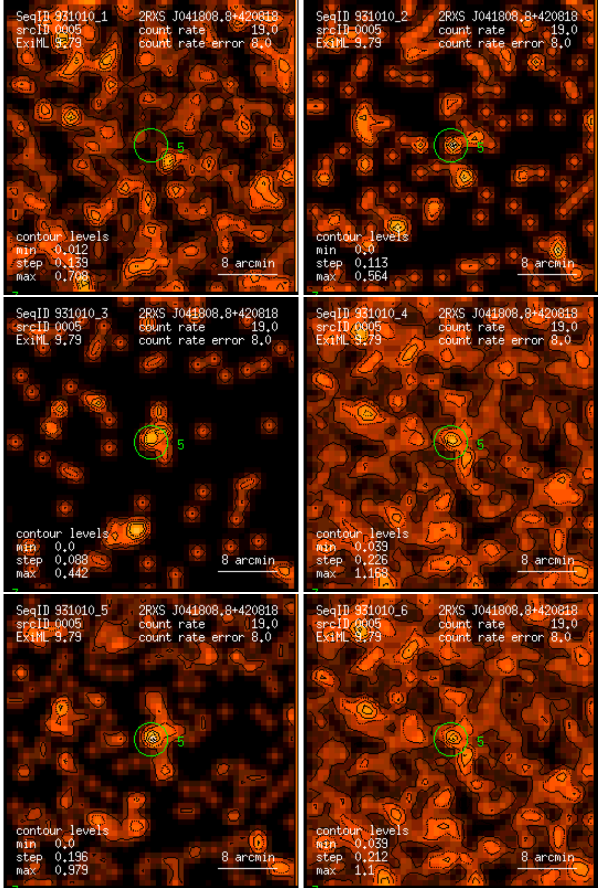
Figure 5: RASS 931010: detection 0005: band rate images, Gaussian filter: (1) PSPC channels 11 – 41, (2) 52 – 90, (3) 91 – 201, (4) 11 – 235, (5) 52 – 201, (6) 11 – 201. Broad band rates in counts/ks. Band rate contour levels in counts/ks/arcmin 2 .
