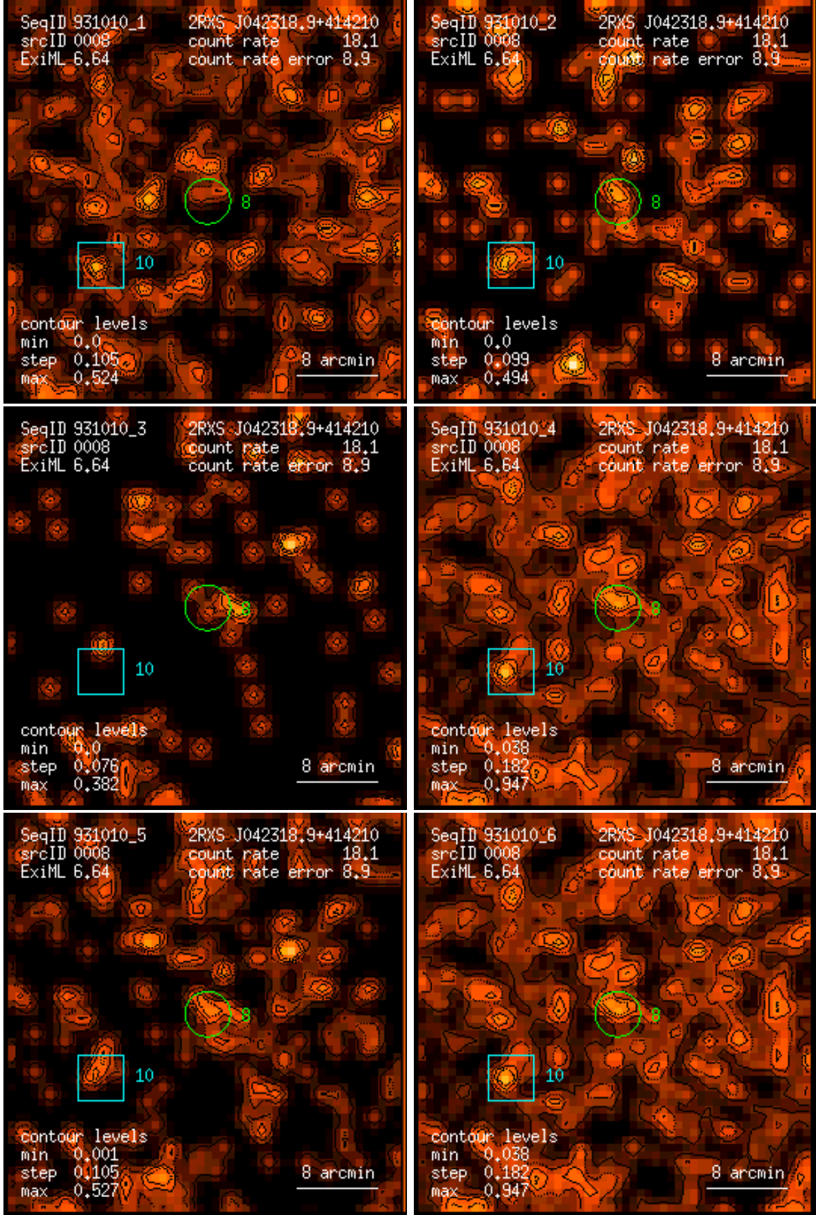
Figure 8: RASS 931010: detection 0008: band rate images, Gaussian filter: (1) PSPC channels 11 – 41, (2) 52 – 90, (3) 91 – 201, (4) 11 – 235, (5) 52 – 201, (6) 11 – 201. Broad band rates in counts/ks. Band rate contour levels in counts/ks/arcmin 2 .
