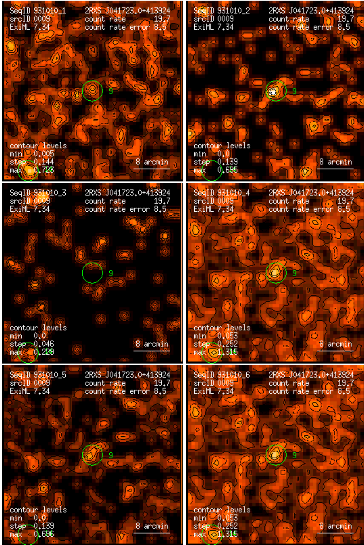
Figure 9: RASS 931010: detection 0009: band rate images, Gaussian filter: (1) PSPC channels 11 – 41, (2) 52 – 90, (3) 91 – 201, (4) 11 – 235, (5) 52 – 201, (6) 11 – 201. Broad band rates in counts/ks. Band rate contour levels in counts/ks/arcmin 2 .
