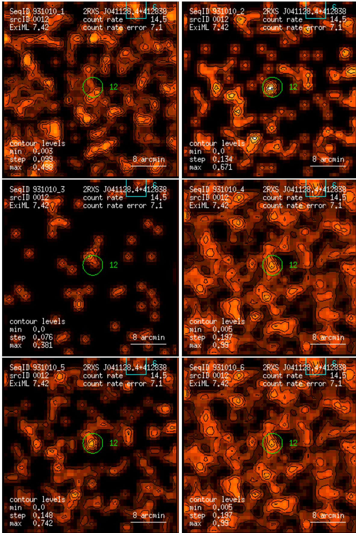
Figure 12: RASS 931010: detection 0012: band rate images, Gaussian filter: (1) PSPC channels 11 – 41, (2) 52 – 90, (3) 91 – 201, (4) 11 – 235, (5) 52 – 201, (6) 11 – 201. Broad band rates in counts/ks. Band rate contour levels in counts/ks/arcmin 2 .
