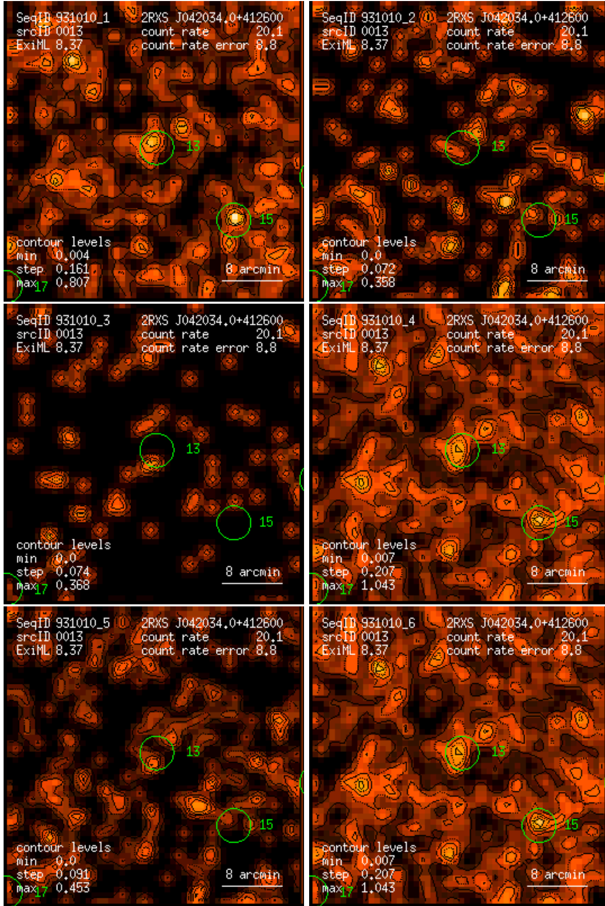
Figure 13: RASS 931010: detection 0013: band rate images, Gaussian filter: (1) PSPC channels 11 – 41, (2) 52 – 90, (3) 91 – 201, (4) 11 – 235, (5) 52 – 201, (6) 11 – 201. Broad band rates in counts/ks. Band rate contour levels in counts/ks/arcmin 2 .
