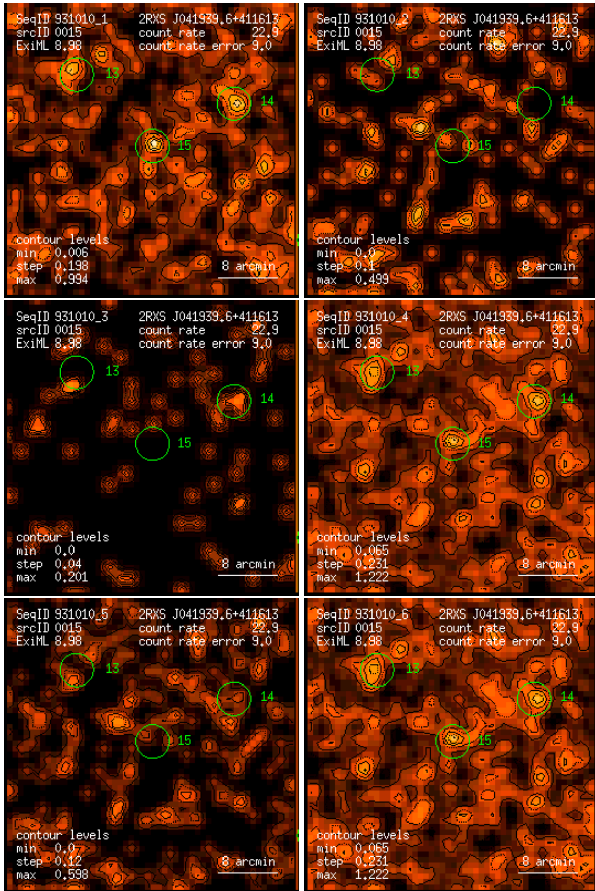
Figure 15: RASS 931010: detection 0015: band rate images, Gaussian filter: (1) PSPC channels 11 – 41, (2) 52 – 90, (3) 91 – 201, (4) 11 – 235, (5) 52 – 201, (6) 11 – 201. Broad band rates in counts/ks. Band rate contour levels in counts/ks/arcmin 2 .
