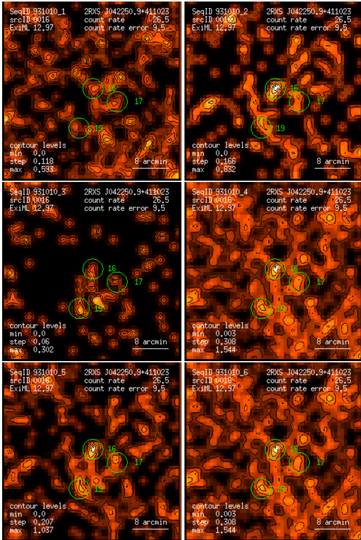
Figure 16: RASS 931010: detection 0016: band rate images, Gaussian filter: (1) PSPC channels 11 – 41, (2) 52 – 90, (3) 91 – 201, (4) 11 – 235, (5) 52 – 201, (6) 11 – 201. Broad band rates in counts/ks. Band rate contour levels in counts/ks/arcmin 2 .
