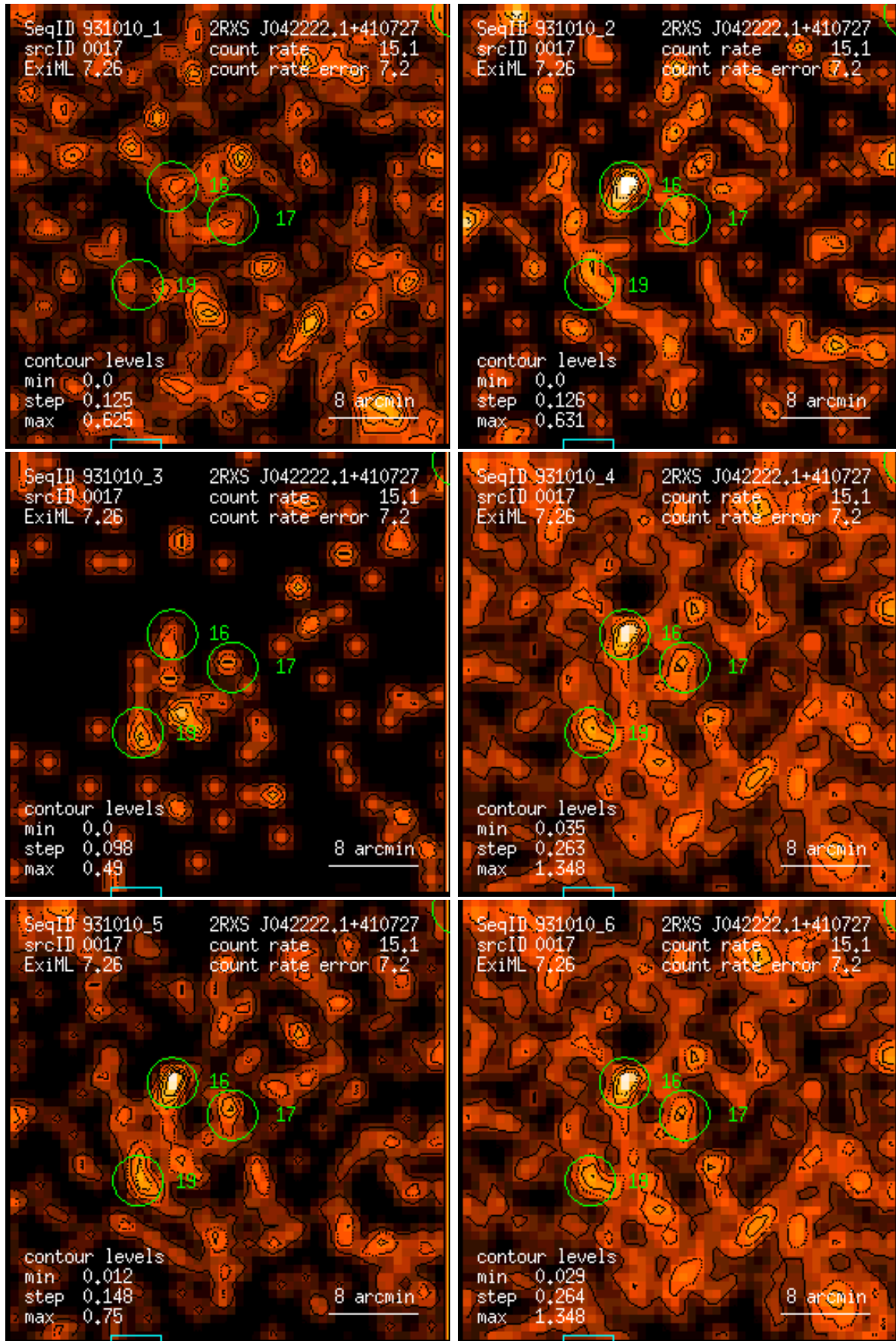
Figure 17: RASS 931010: detection 0017: band rate images, Gaussian filter: (1) PSPC channels 11 – 41, (2) 52 – 90, (3) 91 – 201, (4) 11 – 235, (5) 52 – 201, (6) 11 – 201. Broad band rates in counts/ks. Band rate contour levels in counts/ks/arcmin 2 .
