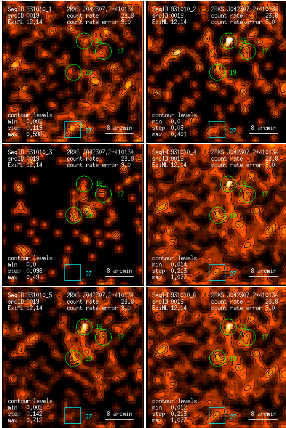
Figure 19: RASS 931010: detection 0019: band rate images, Gaussian filter: (1) PSPC channels 11 – 41, (2) 52 – 90, (3) 91 – 201, (4) 11 – 235, (5) 52 – 201, (6) 11 – 201. Broad band rates in counts/ks. Band rate contour levels in counts/ks/arcmin 2 .
