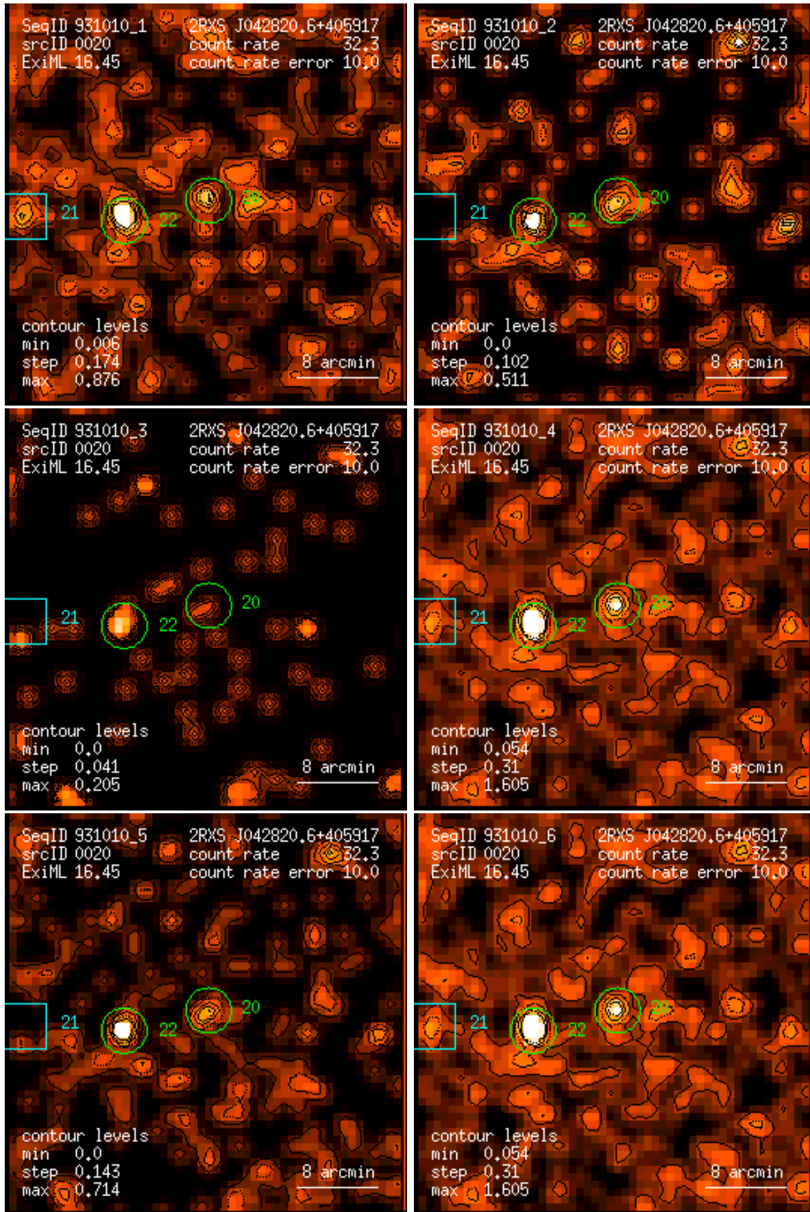
Figure 20: RASS 931010: detection 0020: band rate images, Gaussian filter: (1) PSPC channels 11 – 41, (2) 52 – 90, (3) 91 – 201, (4) 11 – 235, (5) 52 – 201, (6) 11 – 201. Broad band rates in counts/ks. Band rate contour levels in counts/ks/arcmin 2 .
