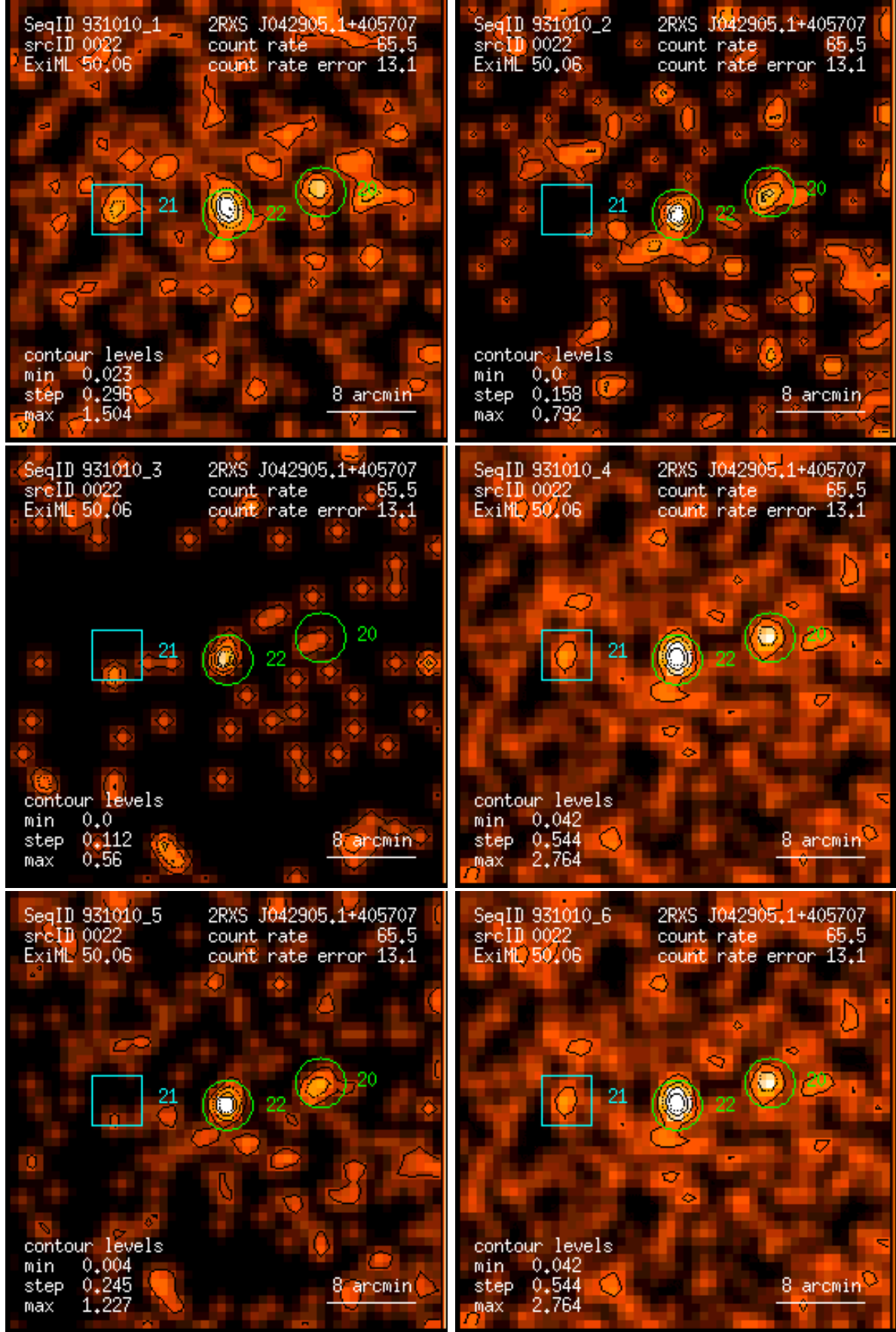
Figure 22: RASS 931010: detection 0022: band rate images, Gaussian filter: (1) PSPC channels 11 – 41, (2) 52 – 90, (3) 91 – 201, (4) 11 – 235, (5) 52 – 201, (6) 11 – 201. Broad band rates in counts/ks. Band rate contour levels in counts/ks/arcmin 2 .
