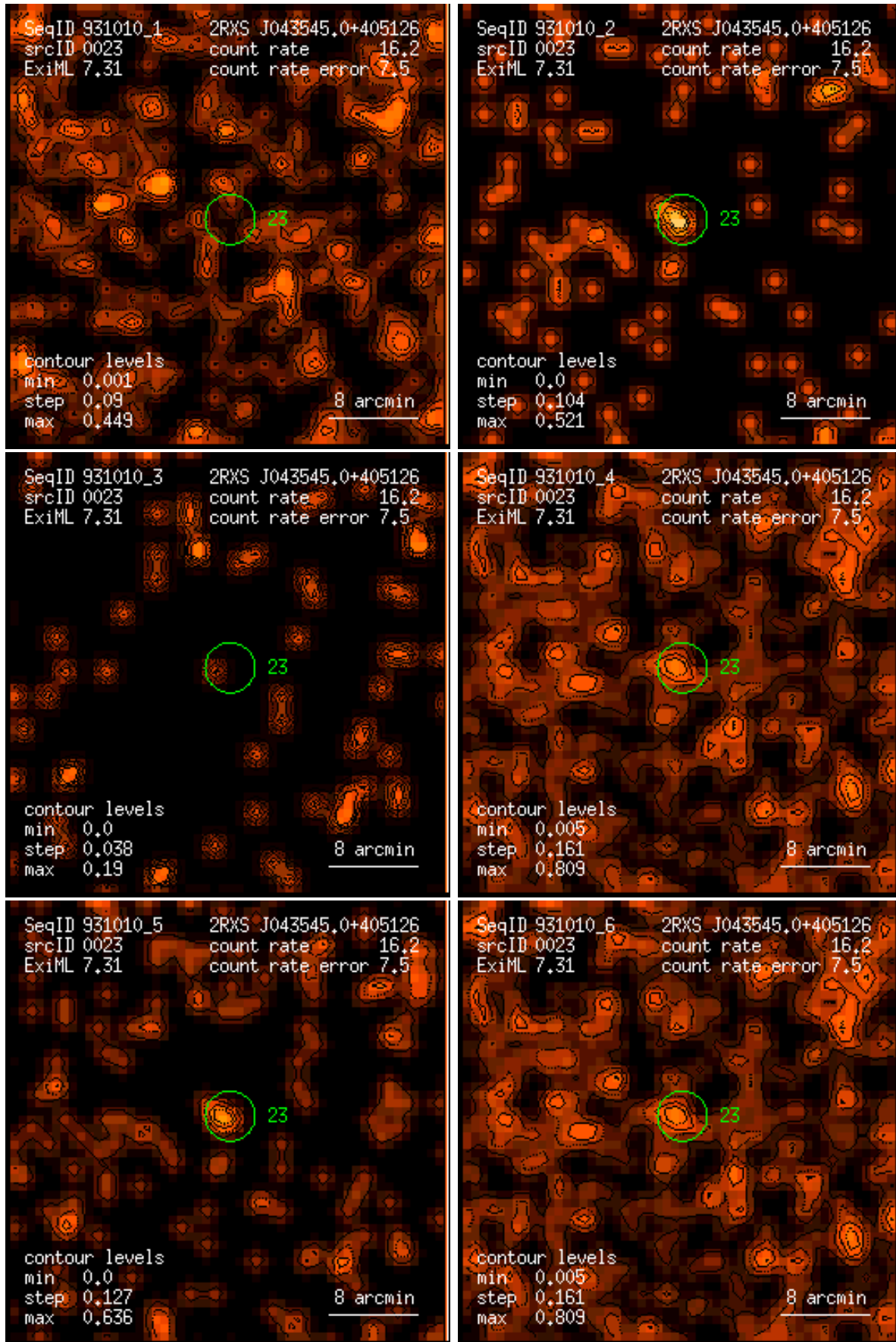
Figure 23: RASS 931010: detection 0023: band rate images, Gaussian filter: (1) PSPC channels 11 – 41, (2) 52 – 90, (3) 91 – 201, (4) 11 – 235, (5) 52 – 201, (6) 11 – 201. Broad band rates in counts/ks. Band rate contour levels in counts/ks/arcmin 2 .
