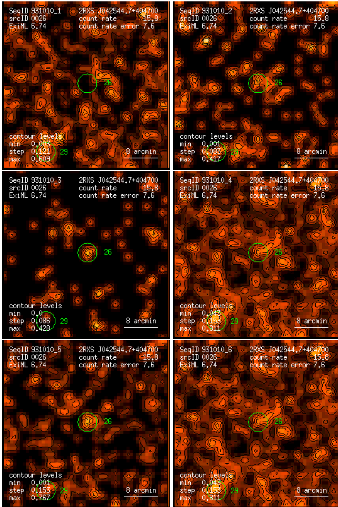
Figure 26: RASS 931010: detection 0026: band rate images, Gaussian filter: (1) PSPC channels 11 – 41, (2) 52 – 90, (3) 91 – 201, (4) 11 – 235, (5) 52 – 201, (6) 11 – 201. Broad band rates in counts/ks. Band rate contour levels in counts/ks/arcmin 2 .
