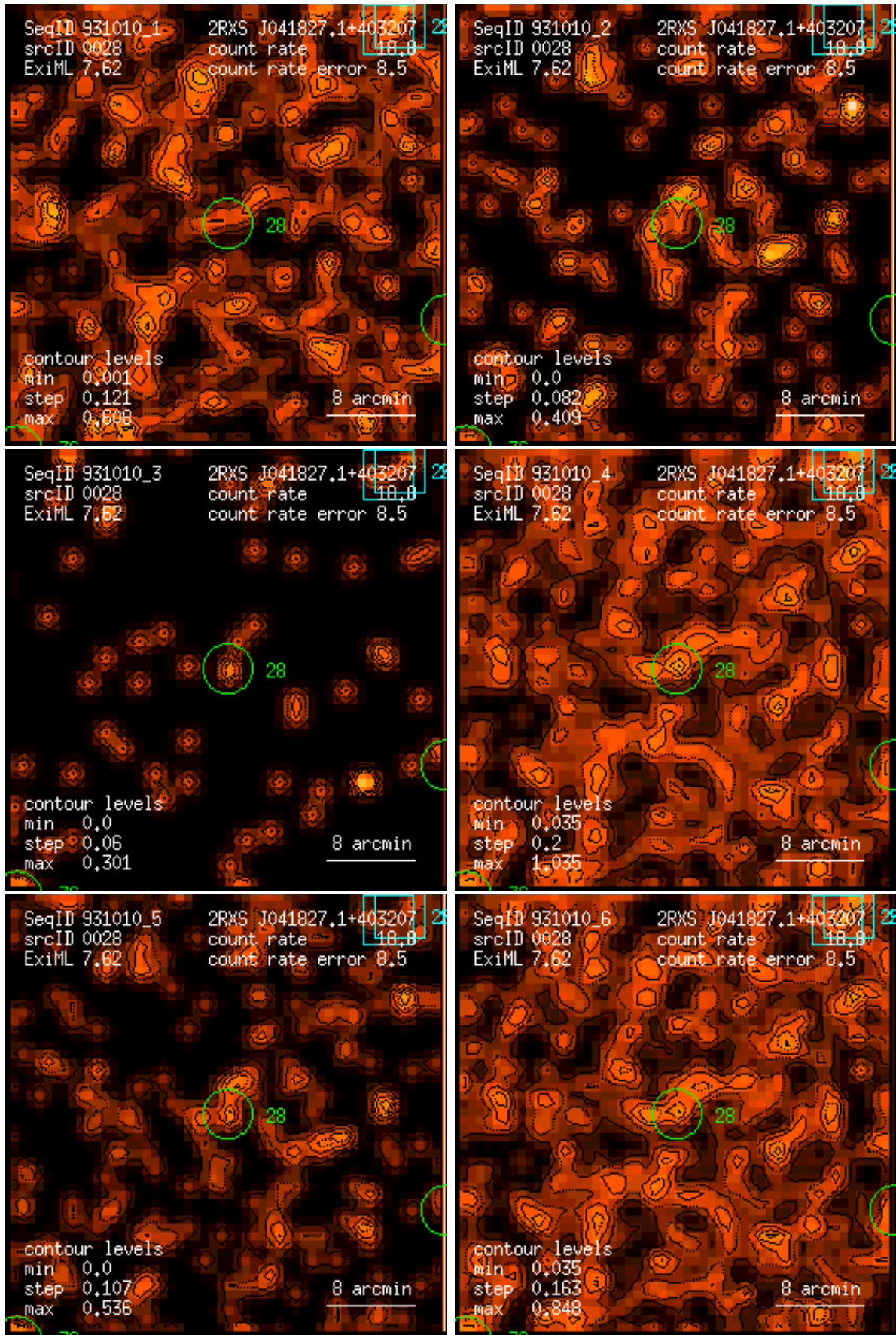
Figure 28: RASS 931010: detection 0028: band rate images, Gaussian filter: (1) PSPC channels 11 – 41, (2) 52 – 90, (3) 91 – 201, (4) 11 – 235, (5) 52 – 201, (6) 11 – 201. Broad band rates in counts/ks. Band rate contour levels in counts/ks/arcmin 2 .
