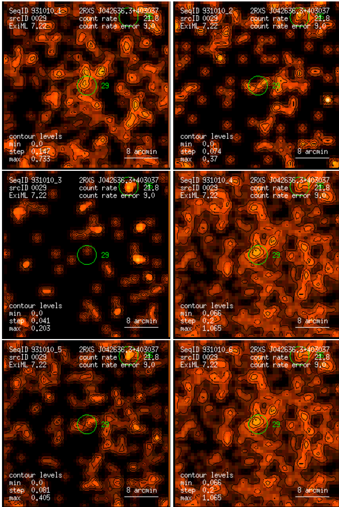
Figure 29: RASS 931010: detection 0029: band rate images, Gaussian filter: (1) PSPC channels 11 – 41, (2) 52 – 90, (3) 91 – 201, (4) 11 – 235, (5) 52 – 201, (6) 11 – 201. Broad band rates in counts/ks. Band rate contour levels in counts/ks/arcmin 2 .
