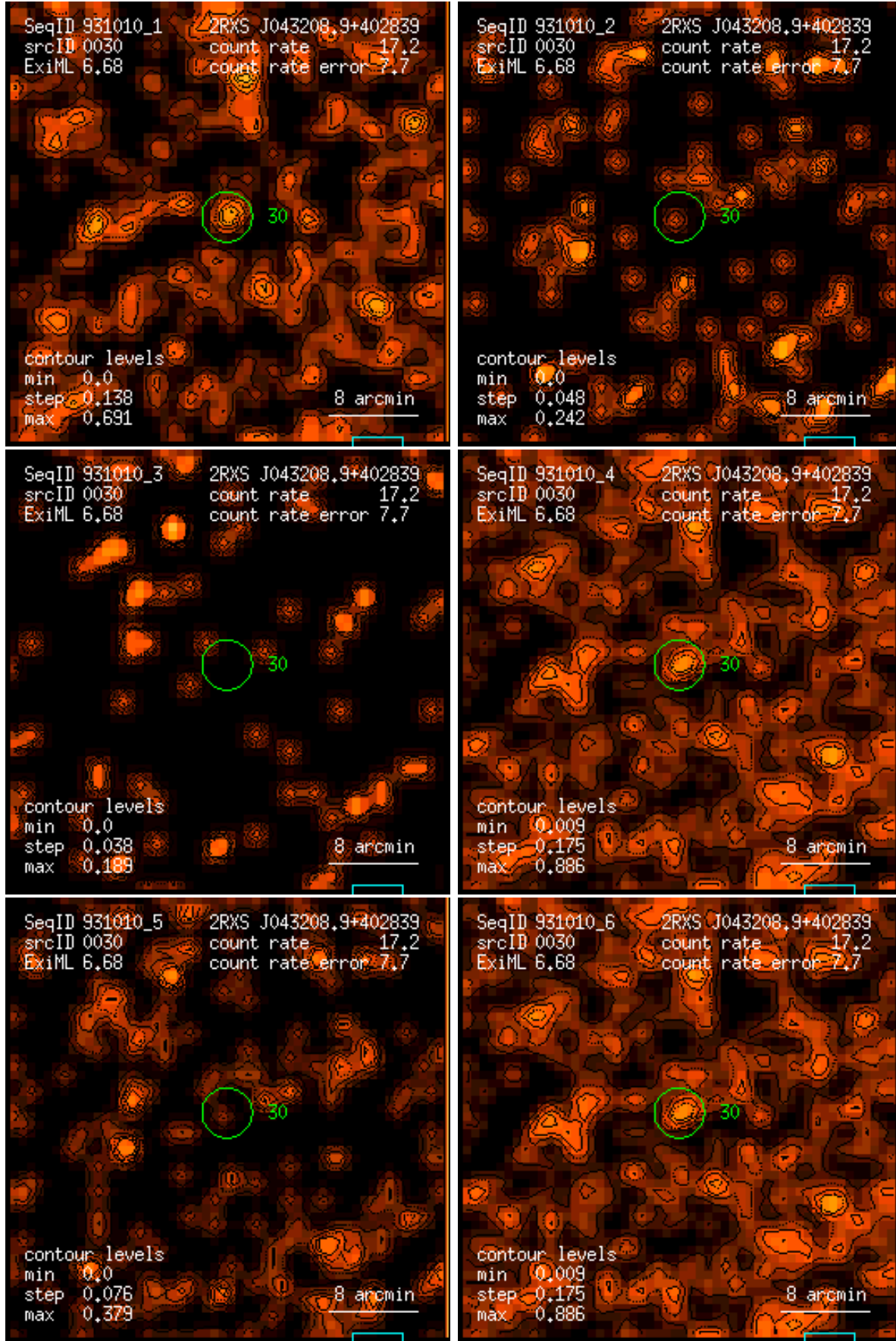
Figure 30: RASS 931010: detection 0030: band rate images, Gaussian filter: (1) PSPC channels 11 – 41, (2) 52 – 90, (3) 91 – 201, (4) 11 – 235, (5) 52 – 201, (6) 11 – 201. Broad band rates in counts/ks. Band rate contour levels in counts/ks/arcmin 2 .
