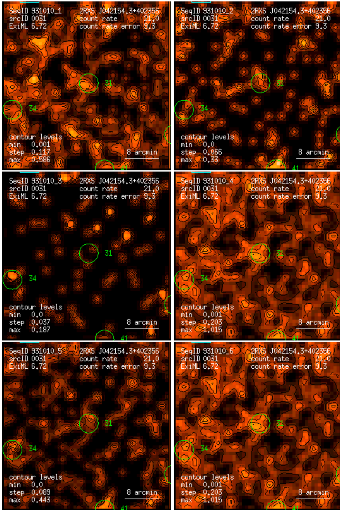
Figure 31: RASS 931010: detection 0031: band rate images, Gaussian filter: (1) PSPC channels 11 – 41, (2) 52 – 90, (3) 91 – 201, (4) 11 – 235, (5) 52 – 201, (6) 11 – 201. Broad band rates in counts/ks. Band rate contour levels in counts/ks/arcmin 2 .
