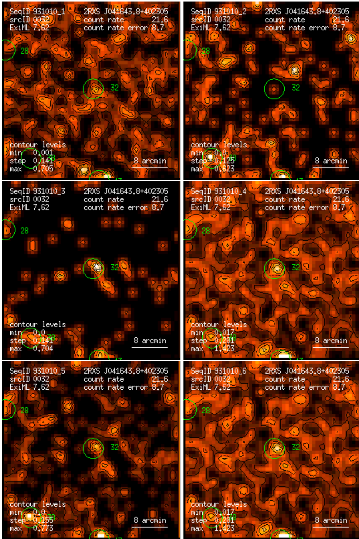
Figure 32: RASS 931010: detection 0032: band rate images, Gaussian filter: (1) PSPC channels 11 – 41, (2) 52 – 90, (3) 91 – 201, (4) 11 – 235, (5) 52 – 201, (6) 11 – 201. Broad band rates in counts/ks. Band rate contour levels in counts/ks/arcmin 2 .
