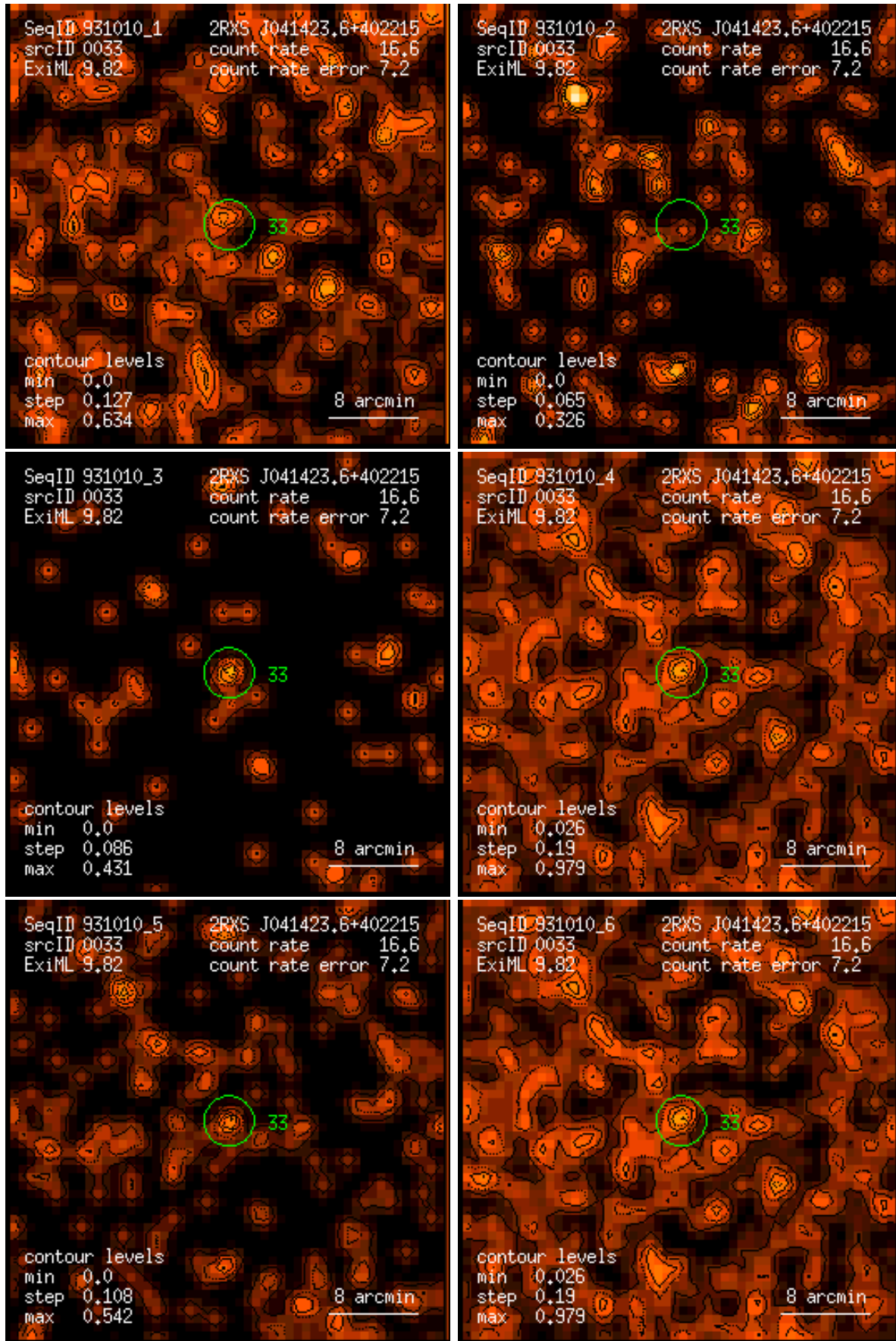
Figure 33: RASS 931010: detection 0033: band rate images, Gaussian filter: (1) PSPC channels 11 – 41, (2) 52 – 90, (3) 91 – 201, (4) 11 – 235, (5) 52 – 201, (6) 11 – 201. Broad band rates in counts/ks. Band rate contour levels in counts/ks/arcmin 2 .
