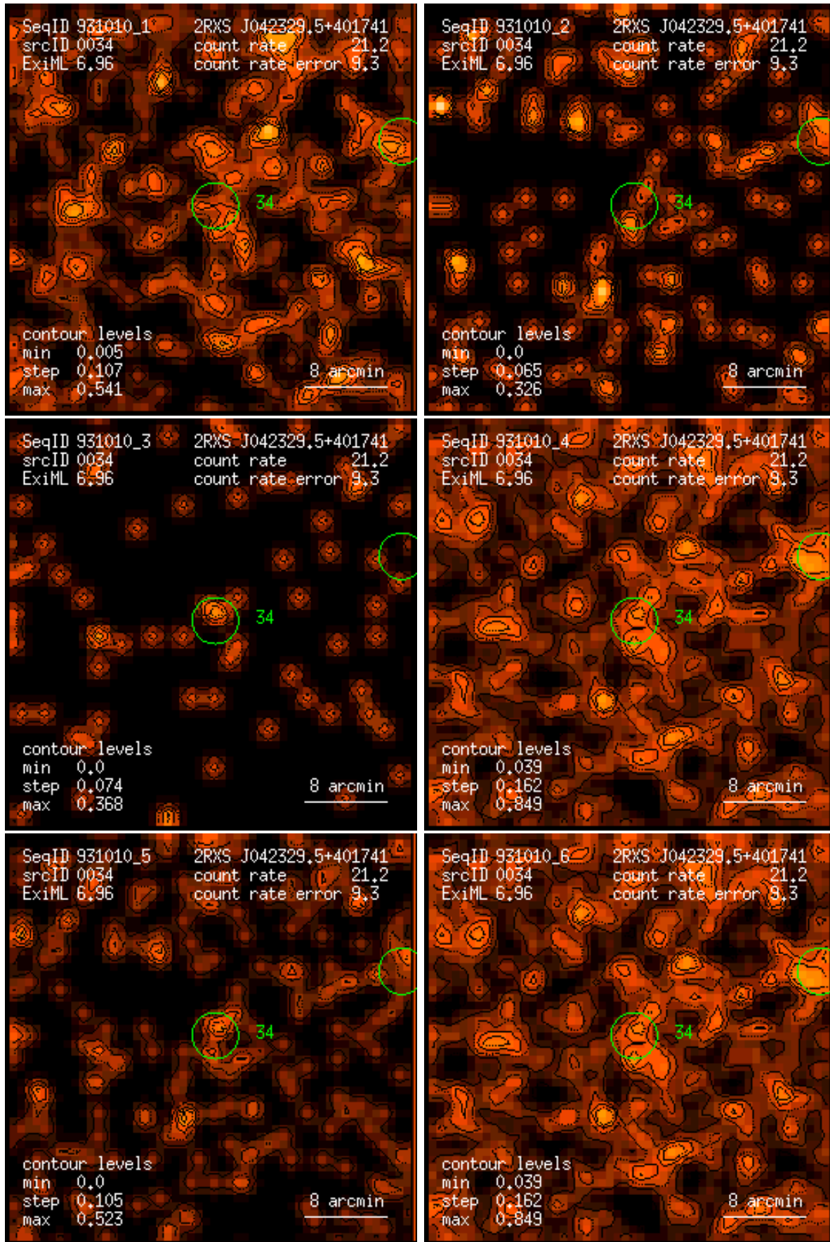
Figure 34: RASS 931010: detection 0034: band rate images, Gaussian filter: (1) PSPC channels 11 – 41, (2) 52 – 90, (3) 91 – 201, (4) 11 – 235, (5) 52 – 201, (6) 11 – 201. Broad band rates in counts/ks. Band rate contour levels in counts/ks/arcmin 2 .
