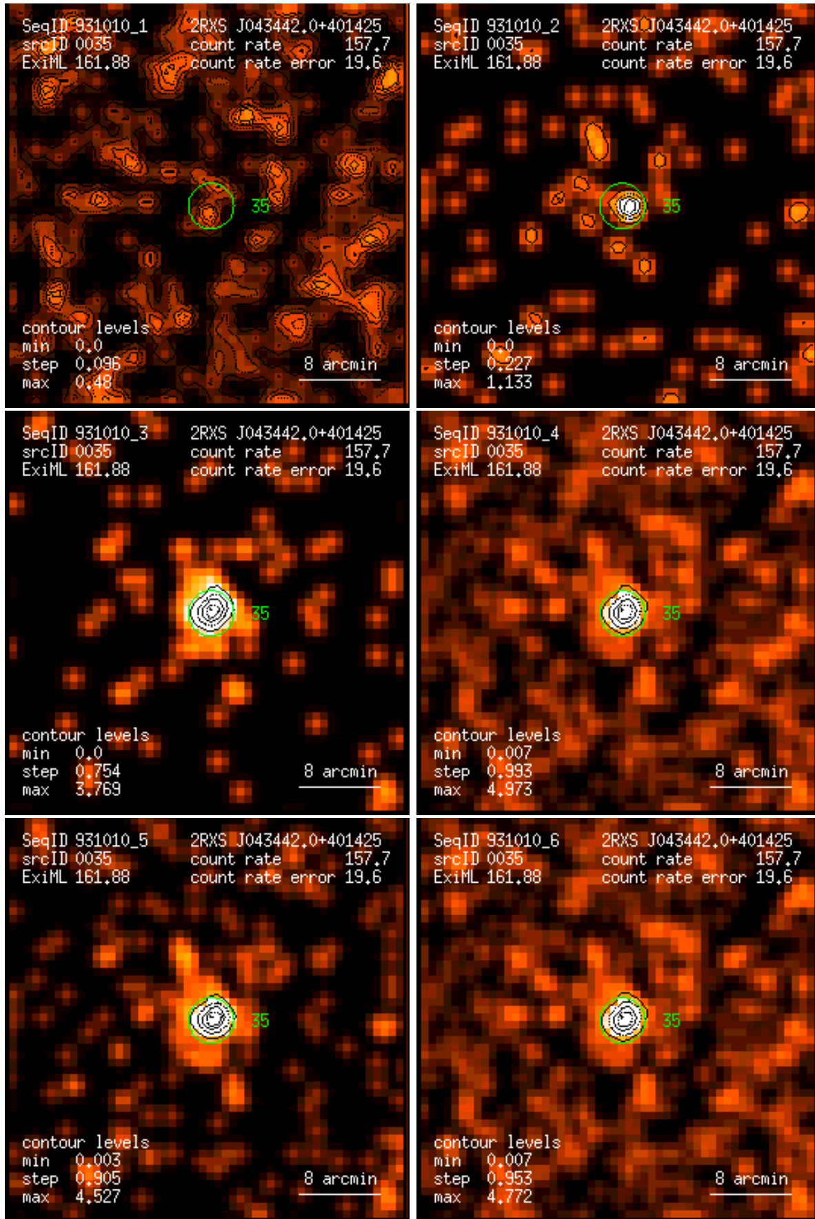
Figure 35: RASS 931010: detection 0035: band rate images, Gaussian filter: (1) PSPC channels 11 – 41, (2) 52 – 90, (3) 91 – 201, (4) 11 – 235, (5) 52 – 201, (6) 11 – 201. Broad band rates in counts/ks. Band rate contour levels in counts/ks/arcmin 2 .
