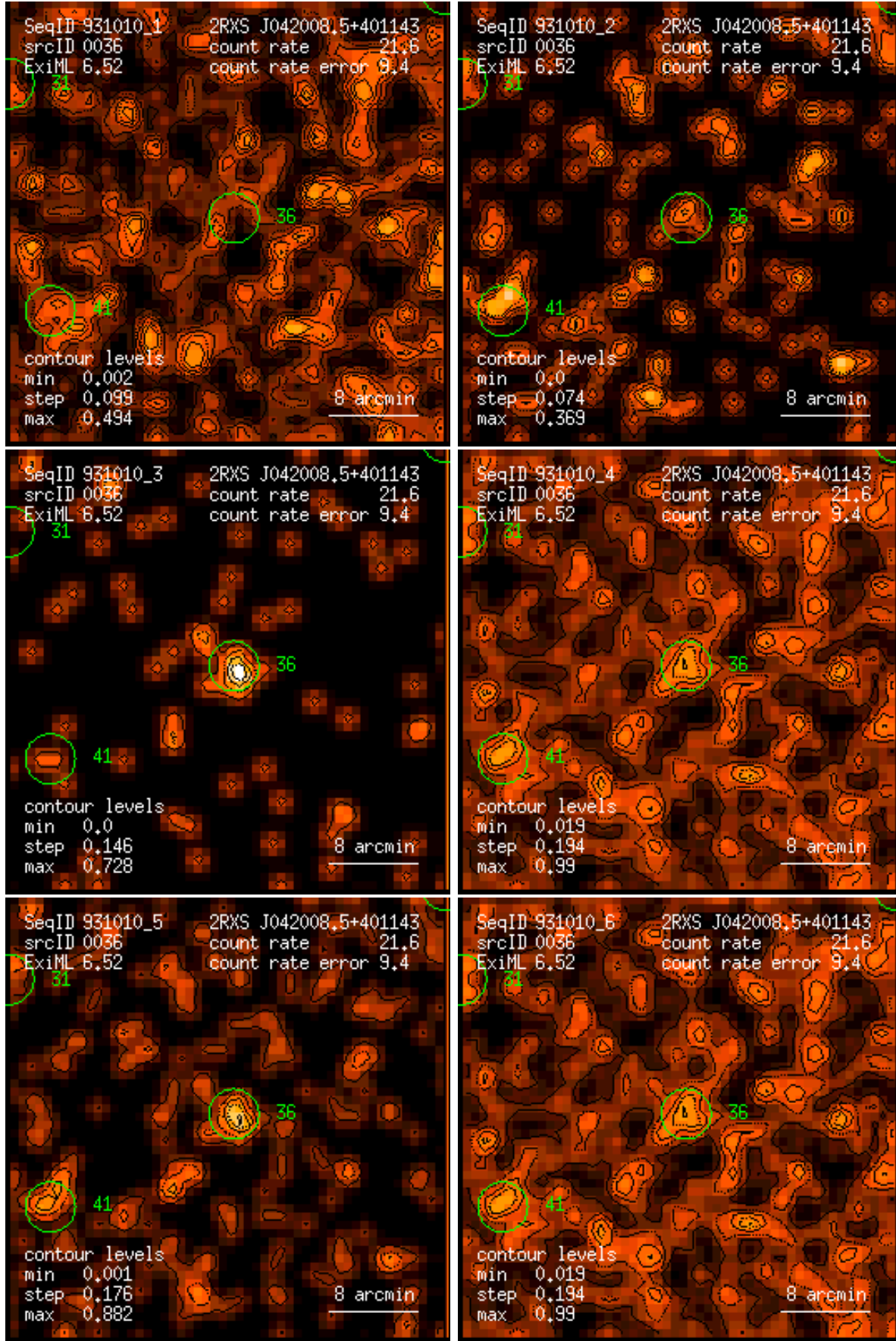
Figure 36: RASS 931010: detection 0036: band rate images, Gaussian filter: (1) PSPC channels 11 – 41, (2) 52 – 90, (3) 91 – 201, (4) 11 – 235, (5) 52 – 201, (6) 11 – 201. Broad band rates in counts/ks. Band rate contour levels in counts/ks/arcmin 2 .
