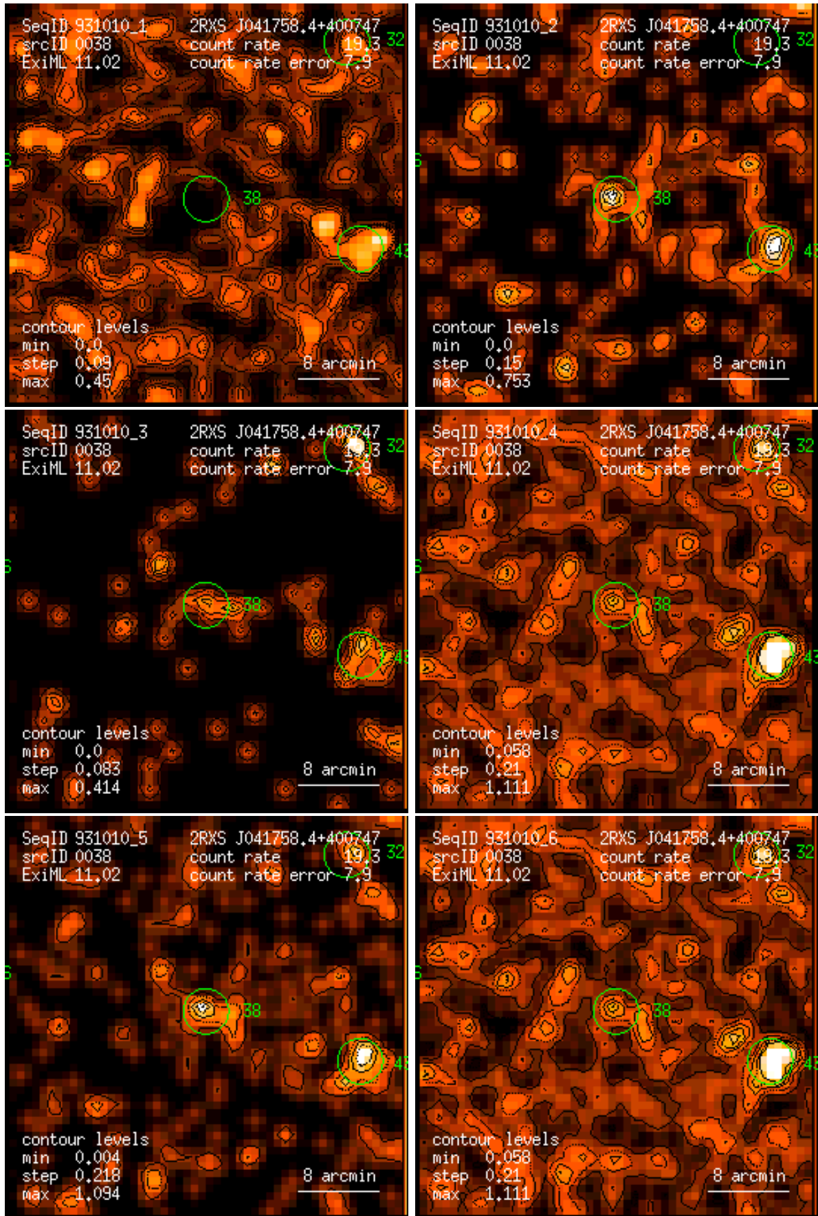
Figure 38: RASS 931010: detection 0038: band rate images, Gaussian filter: (1) PSPC channels 11 – 41, (2) 52 – 90, (3) 91 – 201, (4) 11 – 235, (5) 52 – 201, (6) 11 – 201. Broad band rates in counts/ks. Band rate contour levels in counts/ks/arcmin 2 .
