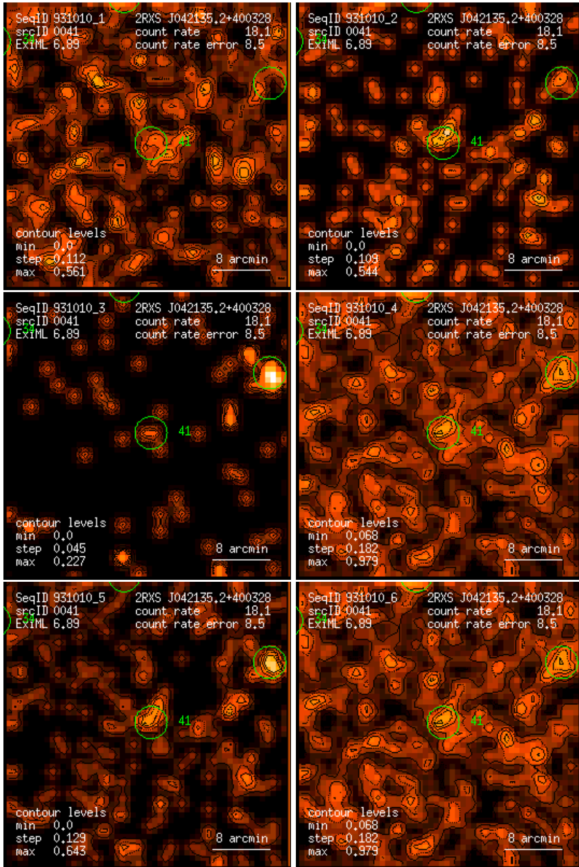
Figure 41: RASS 931010: detection 0041: band rate images, Gaussian filter: (1) PSPC channels 11 – 41, (2) 52 – 90, (3) 91 – 201, (4) 11 – 235, (5) 52 – 201, (6) 11 – 201. Broad band rates in counts/ks. Band rate contour levels in counts/ks/arcmin 2 .
