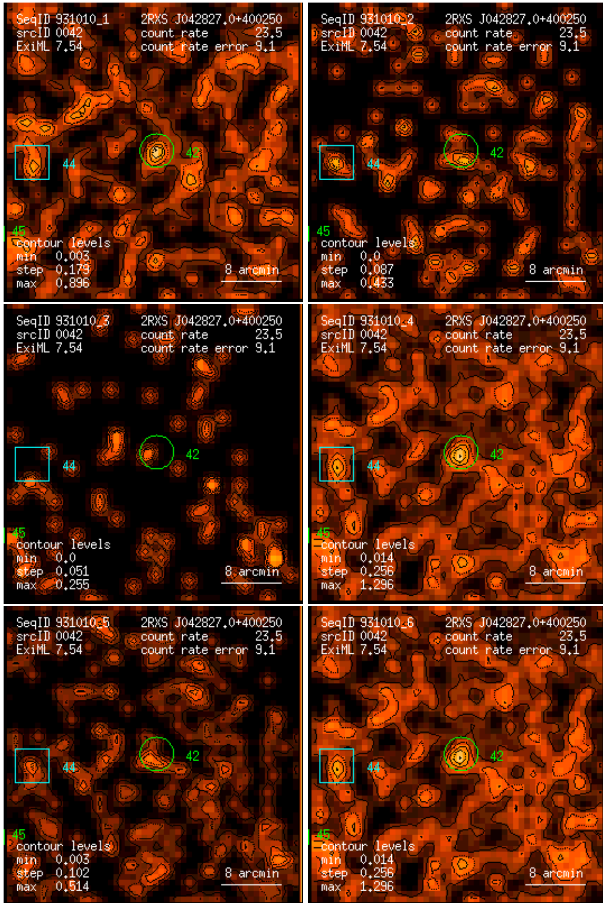
Figure 42: RASS 931010: detection 0042: band rate images, Gaussian filter: (1) PSPC channels 11 – 41, (2) 52 – 90, (3) 91 – 201, (4) 11 – 235, (5) 52 – 201, (6) 11 – 201. Broad band rates in counts/ks. Band rate contour levels in counts/ks/arcmin 2 .
