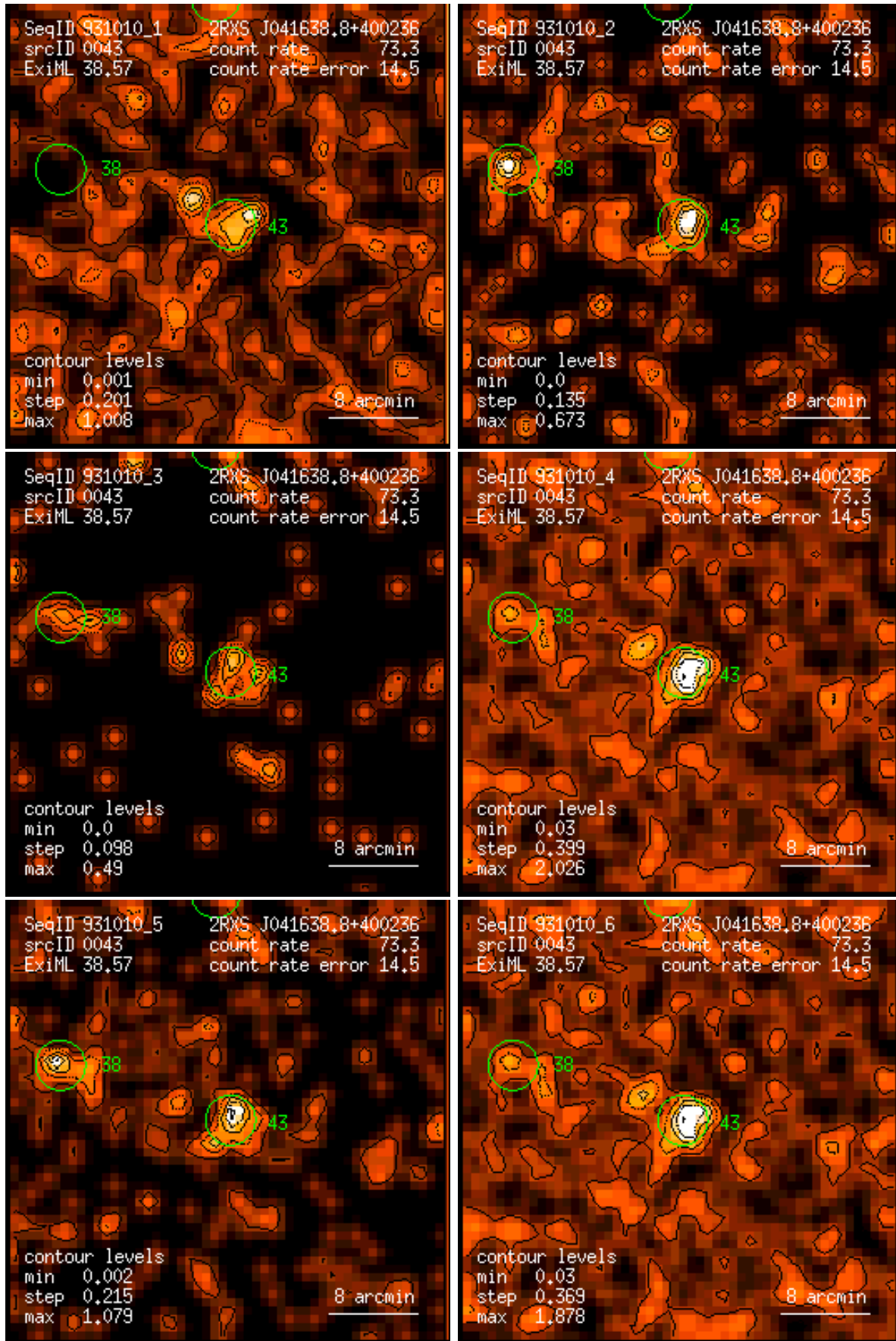
Figure 43: RASS 931010: detection 0043: band rate images, Gaussian filter: (1) PSPC channels 11 – 41, (2) 52 – 90, (3) 91 – 201, (4) 11 – 235, (5) 52 – 201, (6) 11 – 201. Broad band rates in counts/ks. Band rate contour levels in counts/ks/arcmin 2 .
