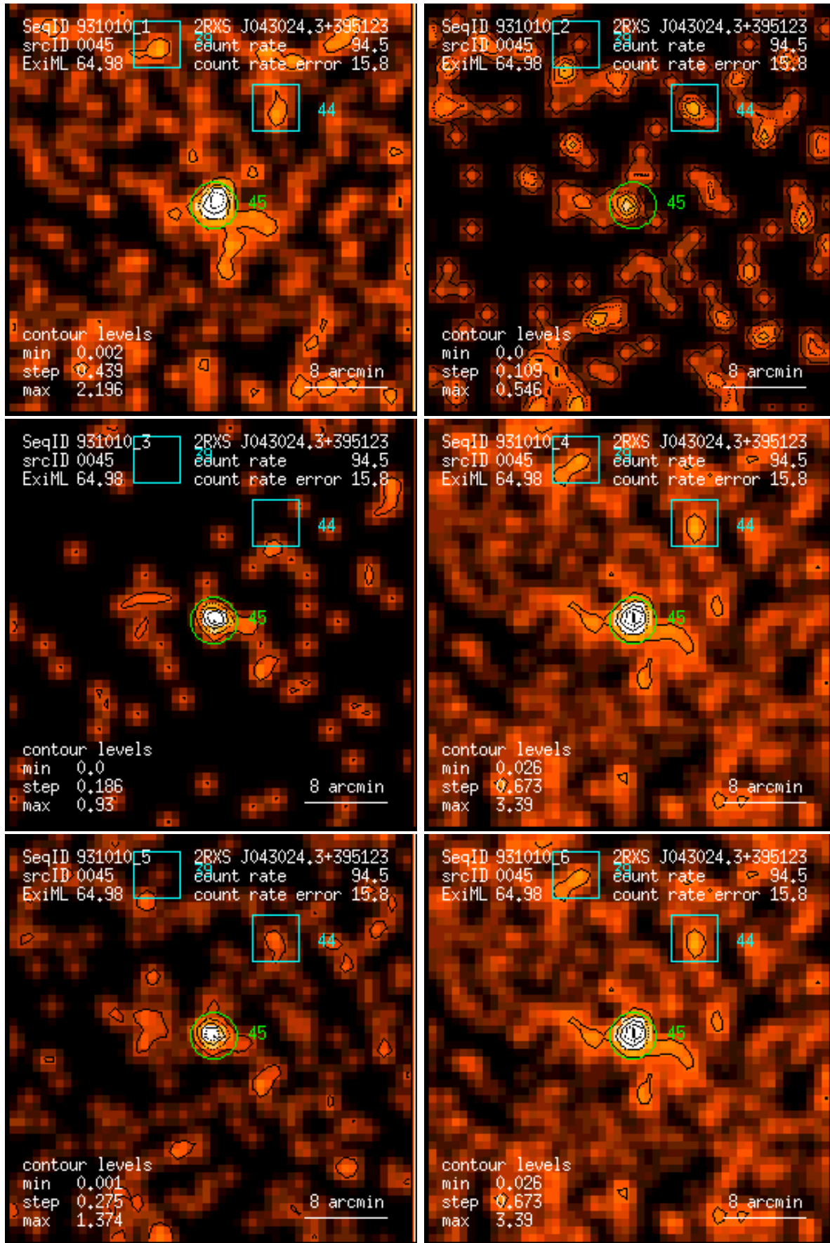
Figure 45: RASS 931010: detection 0045: band rate images, Gaussian filter: (1) PSPC channels 11 – 41, (2) 52 – 90, (3) 91 – 201, (4) 11 – 235, (5) 52 – 201, (6) 11 – 201. Broad band rates in counts/ks. Band rate contour levels in counts/ks/arcmin 2 .
