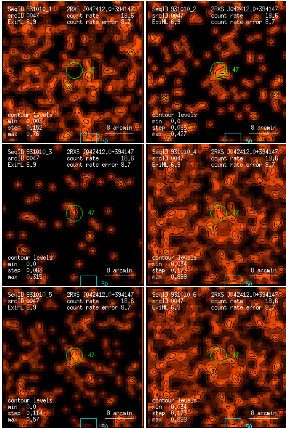
Figure 47: RASS 931010: detection 0047: band rate images, Gaussian filter: (1) PSPC channels 11 – 41, (2) 52 – 90, (3) 91 – 201, (4) 11 – 235, (5) 52 – 201, (6) 11 – 201. Broad band rates in counts/ks. Band rate contour levels in counts/ks/arcmin 2 .
