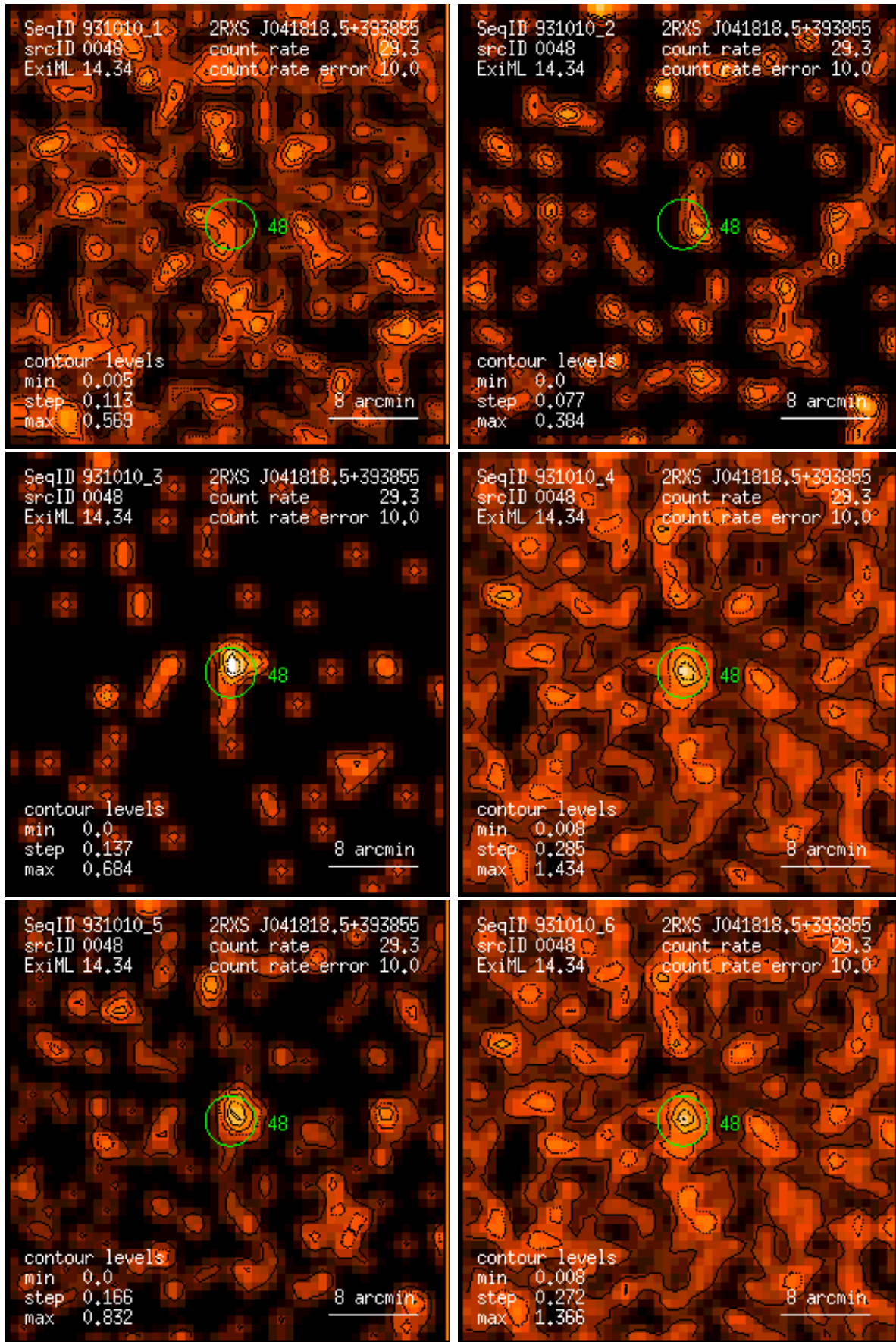
Figure 48: RASS 931010: detection 0048: band rate images, Gaussian filter: (1) PSPC channels 11 – 41, (2) 52 – 90, (3) 91 – 201, (4) 11 – 235, (5) 52 – 201, (6) 11 – 201. Broad band rates in counts/ks. Band rate contour levels in counts/ks/arcmin 2 .
