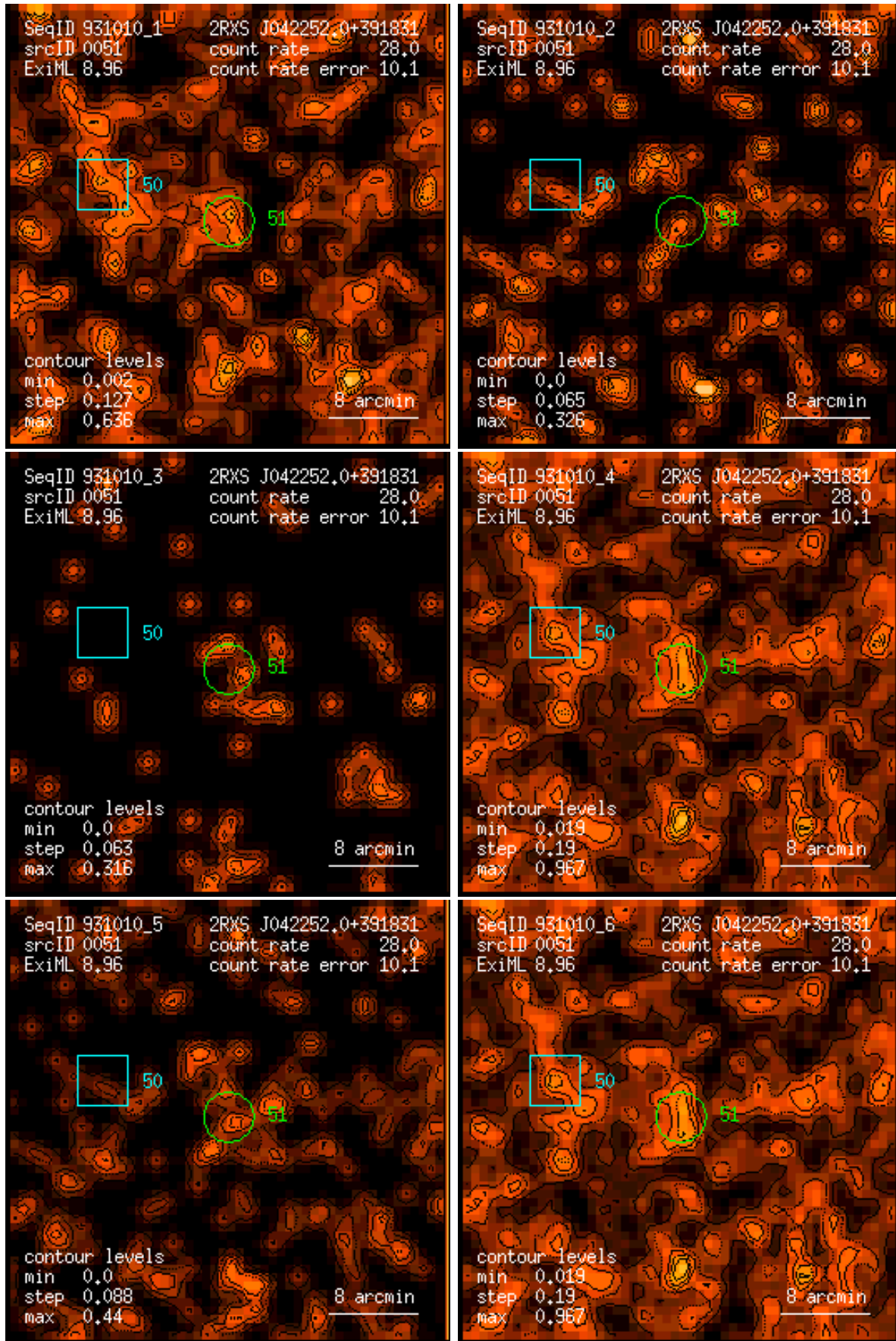
Figure 51: RASS 931010: detection 0051: band rate images, Gaussian filter: (1) PSPC channels 11 – 41, (2) 52 – 90, (3) 91 – 201, (4) 11 – 235, (5) 52 – 201, (6) 11 – 201. Broad band rates in counts/ks. Band rate contour levels in counts/ks/arcmin 2 .
