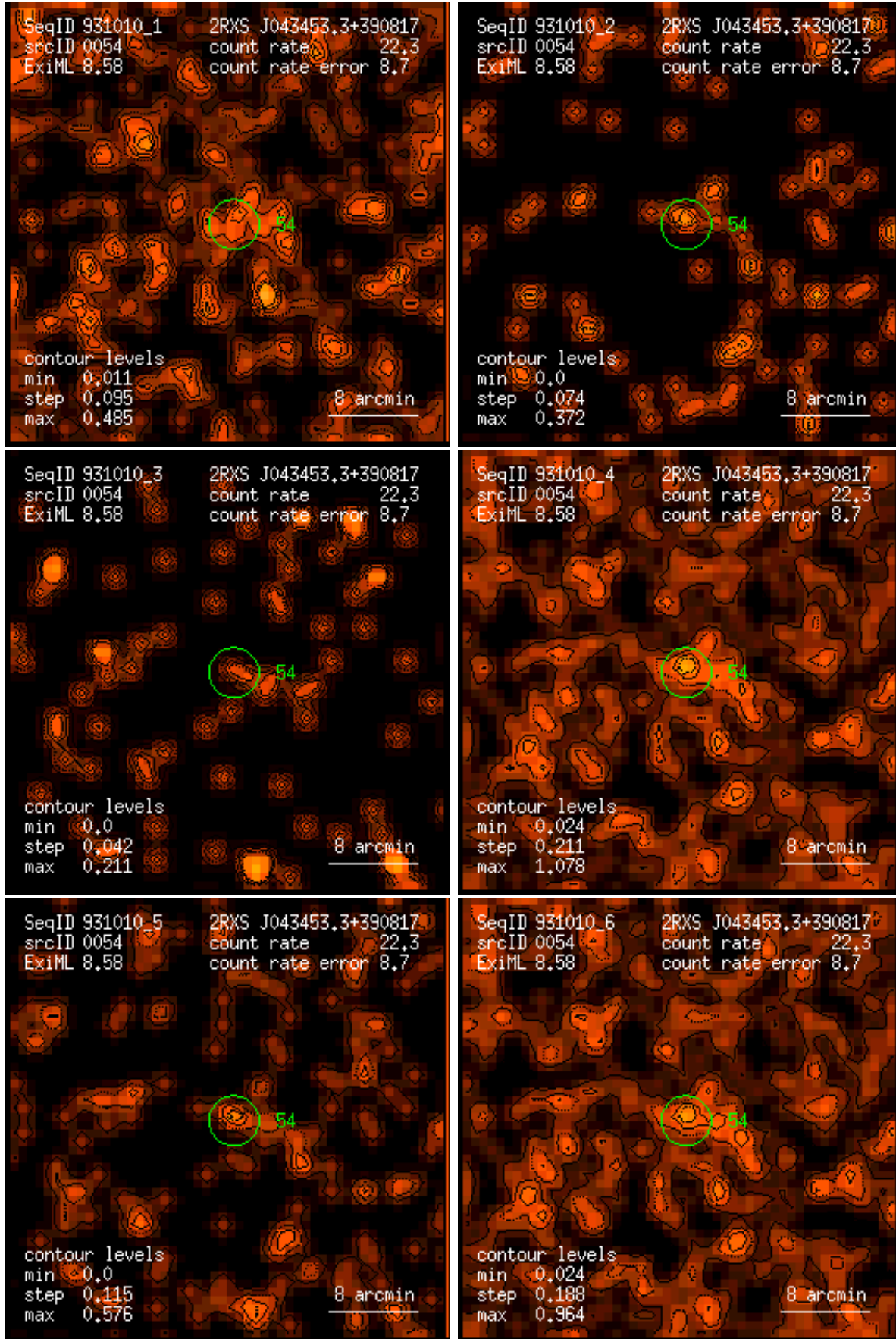
Figure 54: RASS 931010: detection 0054: band rate images, Gaussian filter: (1) PSPC channels 11 – 41, (2) 52 – 90, (3) 91 – 201, (4) 11 – 235, (5) 52 – 201, (6) 11 – 201. Broad band rates in counts/ks. Band rate contour levels in counts/ks/arcmin 2 .
