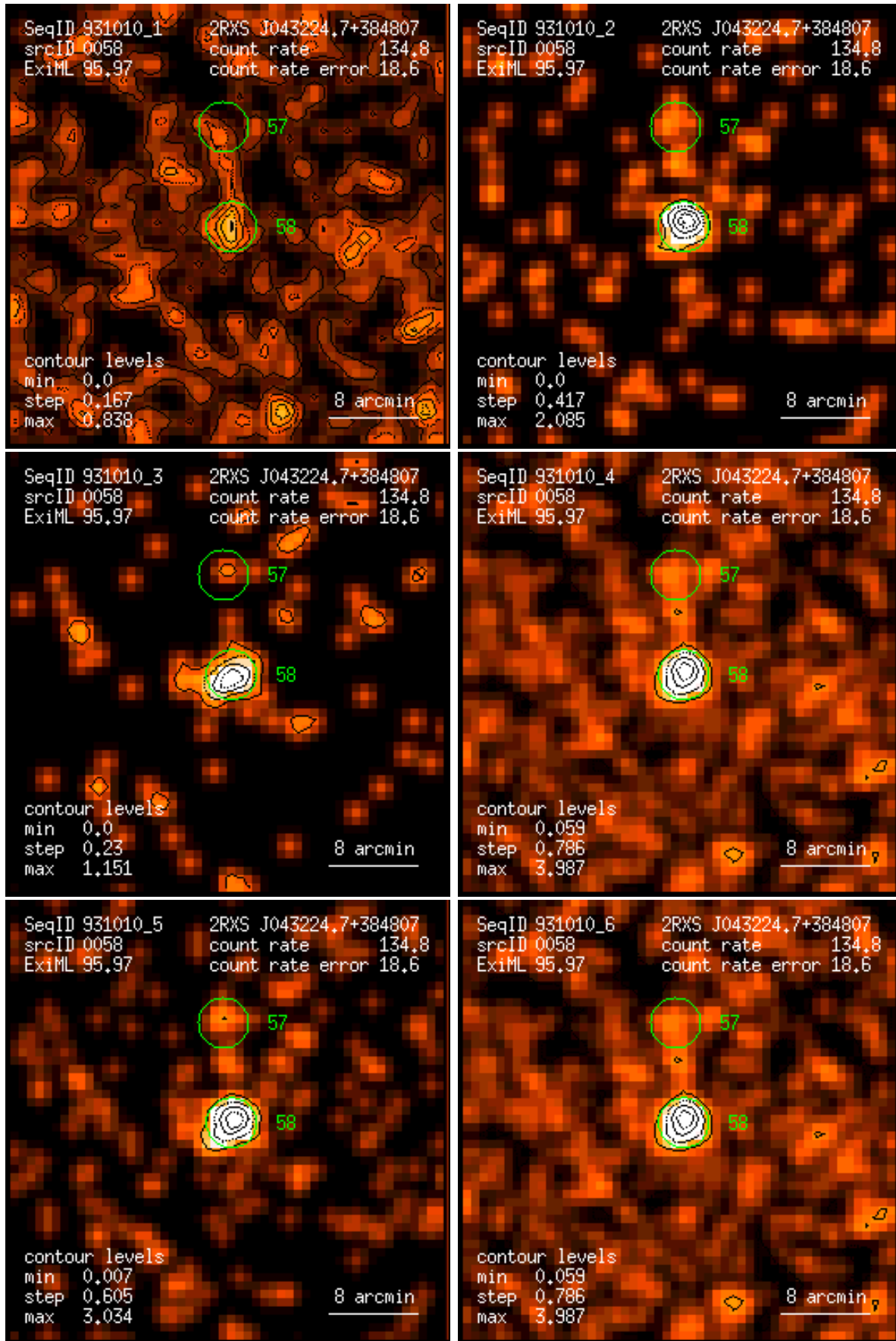
Figure 58: RASS 931010: detection 0058: band rate images, Gaussian filter: (1) PSPC channels 11 – 41, (2) 52 – 90, (3) 91 – 201, (4) 11 – 235, (5) 52 – 201, (6) 11 – 201. Broad band rates in counts/ks. Band rate contour levels in counts/ks/arcmin 2 .
