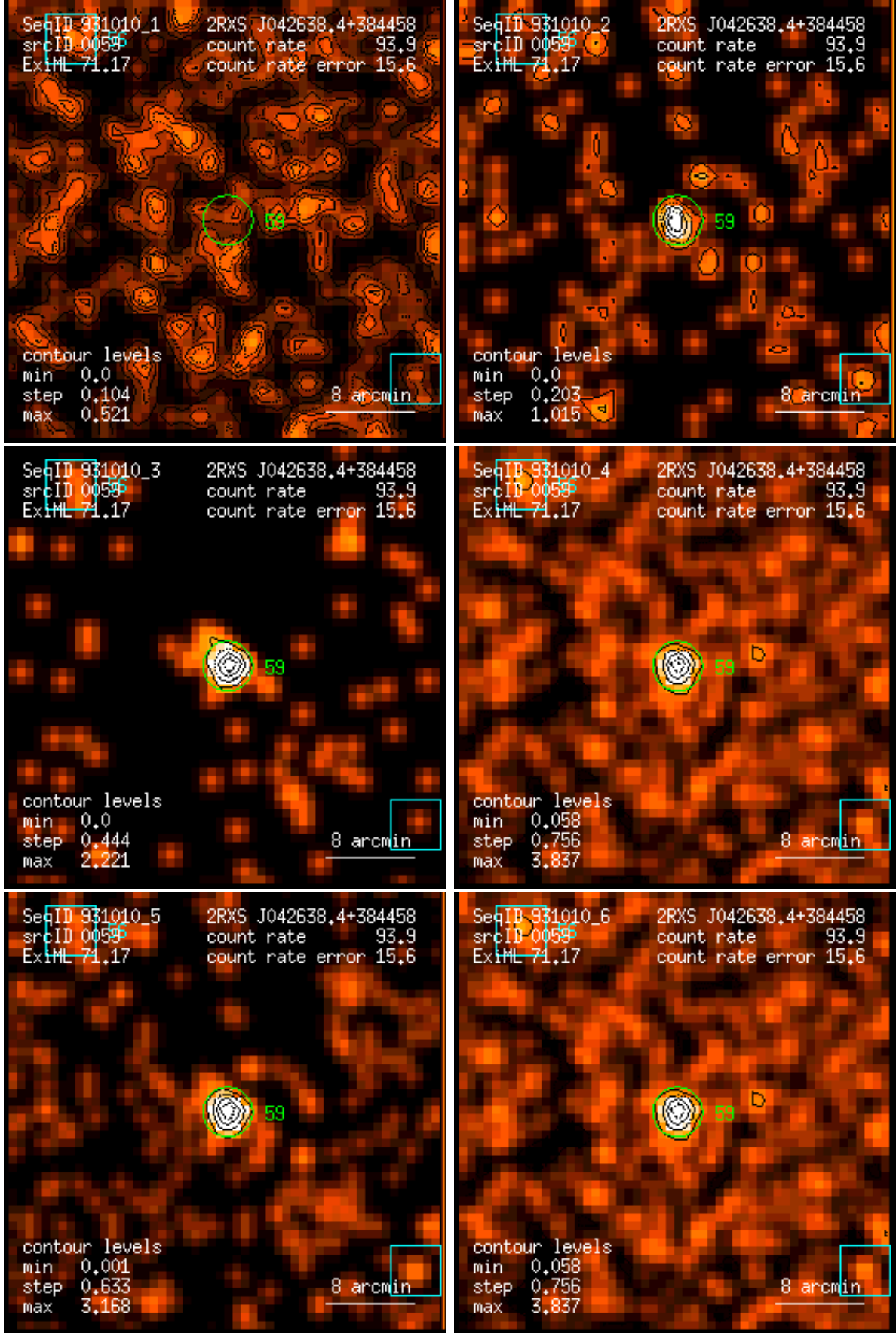
Figure 59: RASS 931010: detection 0059: band rate images, Gaussian filter: (1) PSPC channels 11 – 41, (2) 52 – 90, (3) 91 – 201, (4) 11 – 235, (5) 52 – 201, (6) 11 – 201. Broad band rates in counts/ks. Band rate contour levels in counts/ks/arcmin 2 .
