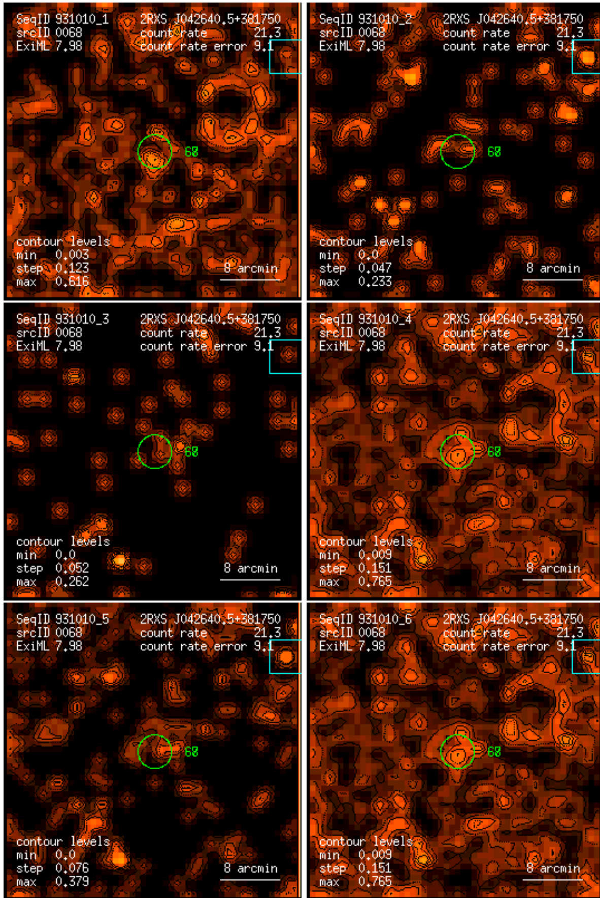
Figure 68: RASS 931010: detection 0068: band rate images, Gaussian filter: (1) PSPC channels 11 – 41, (2) 52 – 90, (3) 91 – 201, (4) 11 – 235, (5) 52 – 201, (6) 11 – 201. Broad band rates in counts/ks. Band rate contour levels in counts/ks/arcmin 2 .
