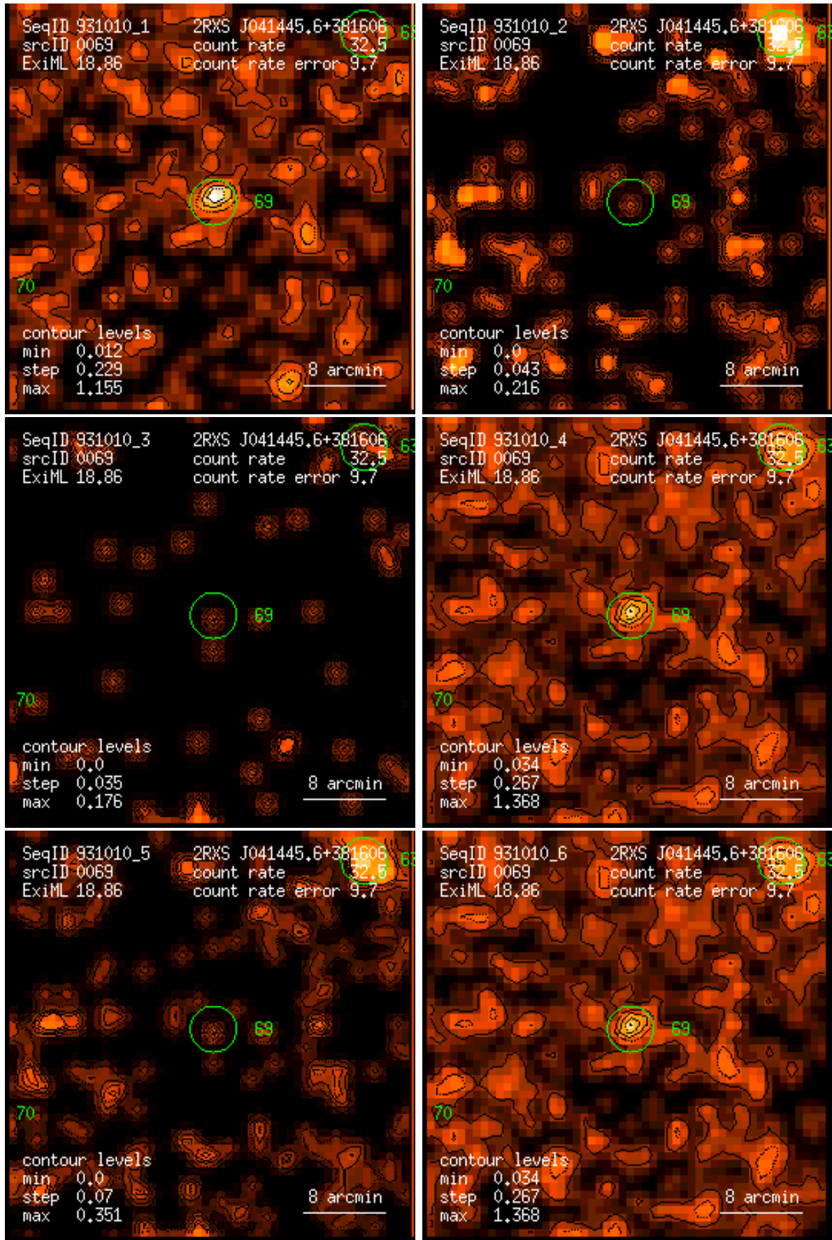
Figure 69: RASS 931010: detection 0069: band rate images, Gaussian filter: (1) PSPC channels 11 – 41, (2) 52 – 90, (3) 91 – 201, (4) 11 – 235, (5) 52 – 201, (6) 11 – 201. Broad band rates in counts/ks. Band rate contour levels in counts/ks/arcmin 2 .
