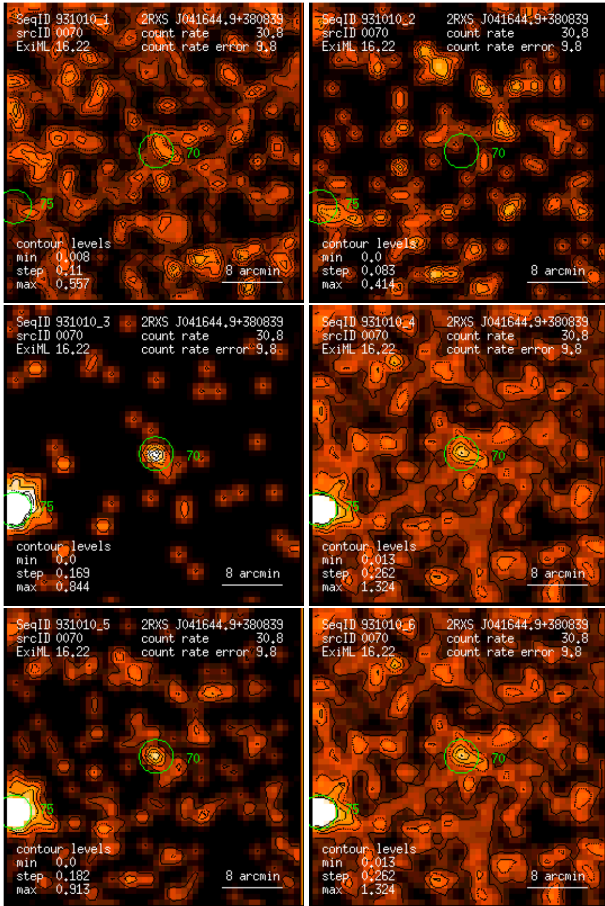
Figure 70: RASS 931010: detection 0070: band rate images, Gaussian filter: (1) PSPC channels 11 – 41, (2) 52 – 90, (3) 91 – 201, (4) 11 – 235, (5) 52 – 201, (6) 11 – 201. Broad band rates in counts/ks. Band rate contour levels in counts/ks/arcmin 2 .
